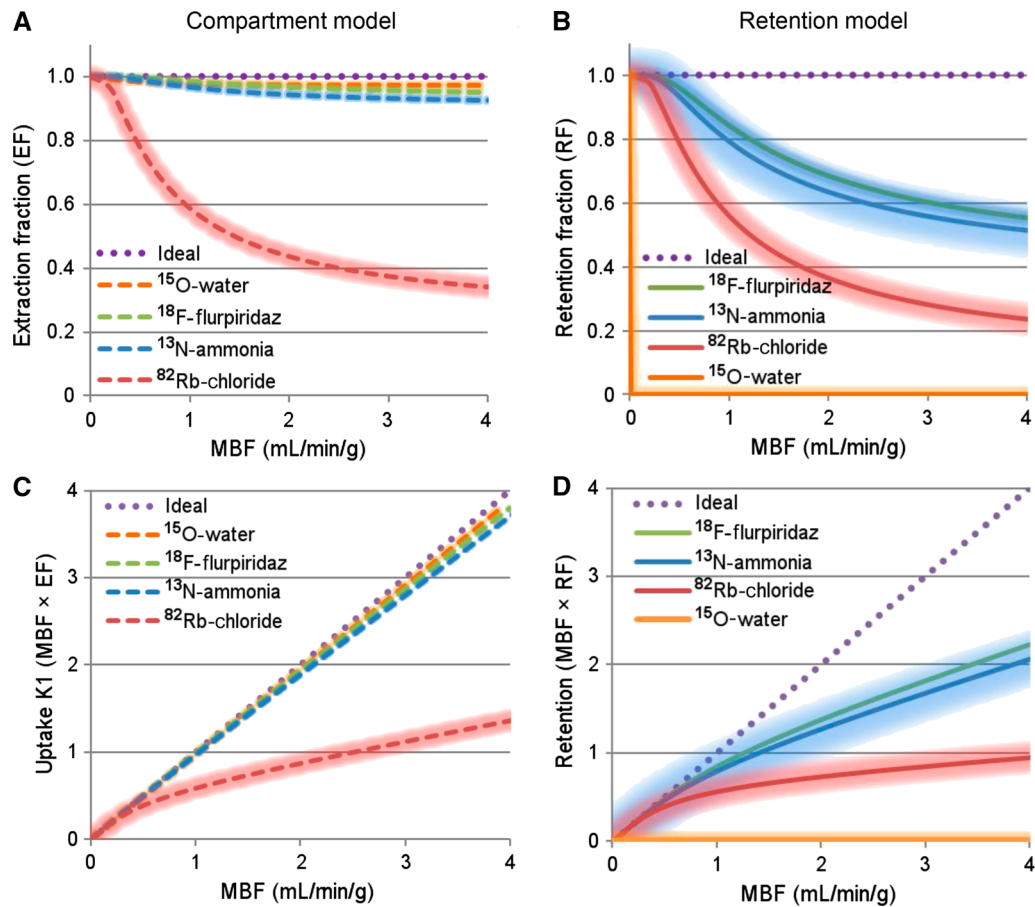
Figure 1. Radiotracer unidirectional extraction fractions (A) used with compartmental modeling of tracer uptake rates K_1 (C), and radiotracer retention fractions (B) used with simplified retention modeling of tracer net uptake (D). Underlying data were obtained from previous publications. 14,22,221,228,229 Limited data suggest that properties of ^{18}F -flurpiridaz are similar to those of ^{13}N -ammonia. Shaded regions represent variability in reported values.
