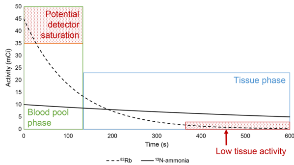
Figure 3. Decay of typical 370-MBq (10 mCi) dose of ^{13}\text{N} -ammonia (solid black line) and 1,665-MBq (45 mCi) dose of ^{82}\text{Rb} (dash line). Because of the ultrashort half-life of ^{82}\text{Rb} , higher activities must be administered to ensure reasonable counting rates during delayed tissue-phase imaging (blue region) for generation of gated and static images for MPI interpretation. However, this results in high counting rates during blood-pool phase (green region) and the potential for detector saturation. Actual threshold for detector saturation will vary with scanner performance.
