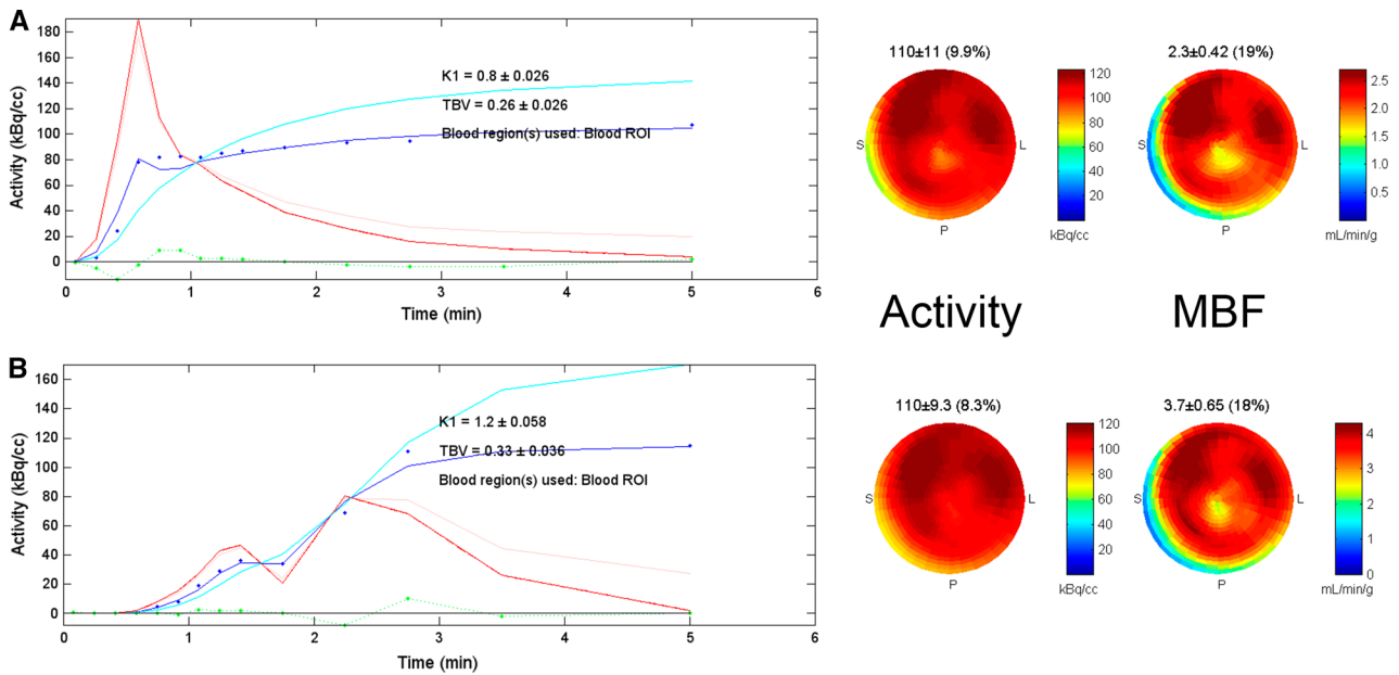
Figure 5. Test-retest dynamic ^{82}\text{Rb} PET MBF scans acquired at 3 and 13 minute after dipyridamole stress. Typical injection profile (A) is shown with single peak of blood input curve (red) at \sim 30 s after scan start time. Poor-quality injection profile (B) shows delayed rise and double-peak of blood input curve, suggesting partial obstruction of intravenous line during tracer administration. Tracer uptake curves (dark blue) and polar maps (activity) are similar after 3–6 min, suggesting that full ^{82}\text{Rb} dose was eventually delivered. However, inconsistent curve shapes result in markedly different MBF estimates (3.7 vs. 2.3 mL/minute/g), as derived from blood-pool-spillover- and partial-volume-corrected tissue curves (cyan).
