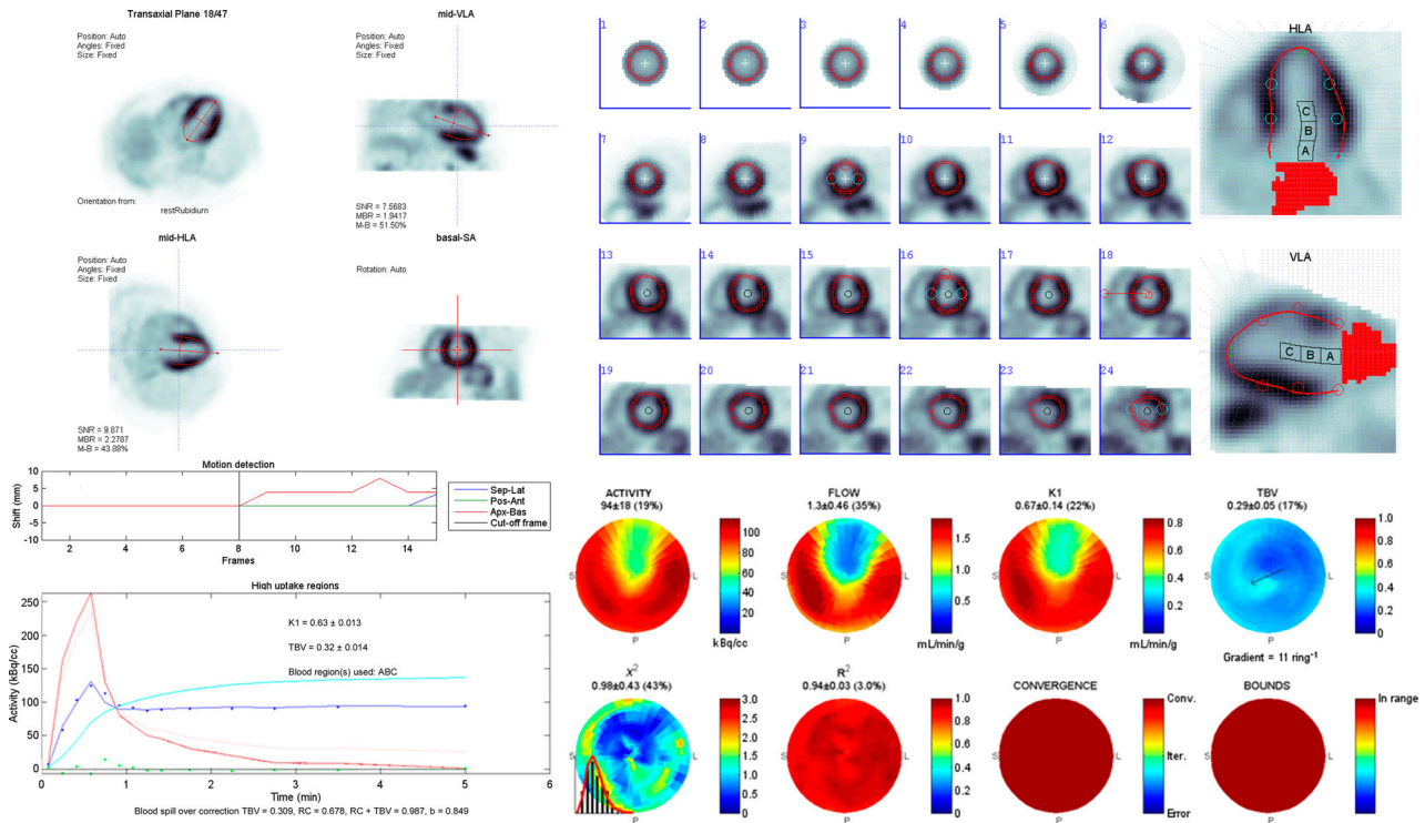
Figure 4. Example ^{82}\text{Rb} stress PET study quality assurance for PET quantification of MBF, including orientation of left ventricular long axis (A), sampling of myocardium and arterial blood regions (B), motion detection, dynamic time–activity curves and kinetic modeling curve-fit (C), regional MBF (FLOW) and total blood volume (TBV) maps, as well as \chi^2 and R^2 goodness-of-fit metrics (D).
