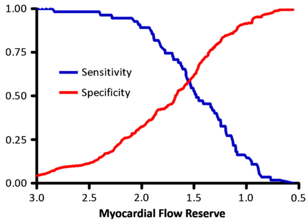
Figure 7. Receiver-operator characteristic curves for detection of severe CAD using MFR. As the threshold for abnormal MFR is decreased from 3.0 to 0.5, sensitivity for high-risk CAD (2-vessel disease including proximal left anterior descending artery, 3-vessel disease, and left main coronary artery) decreases (blue line). Conversely, with lower thresholds for defining abnormal MFR, specificity progressively increases (red line). (Adapted from Naya et al. 91 ).
