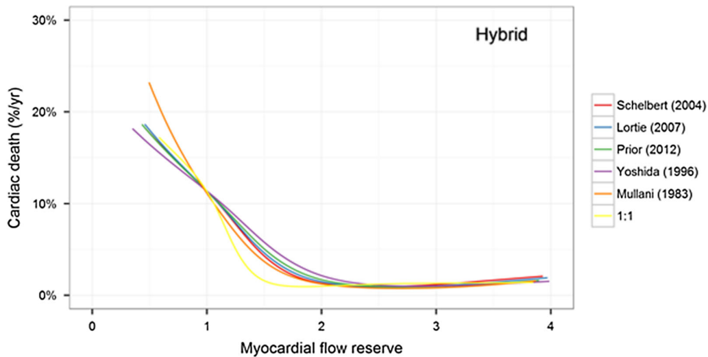
Figure 8. Relationship between MFR and risk of cardiac death. Regardless of which ^{82}\text{Rb} tracer kinetic model is used, similar pattern of rising risk with \text{MFR} < 2 is seen. 1:1 indicates fictitious 100% extraction ( \text{MBF} = K_1 ), which approximates assumptions for myocardial perfusion reserve index. (Adapted from Murthy et al. 54 ).
