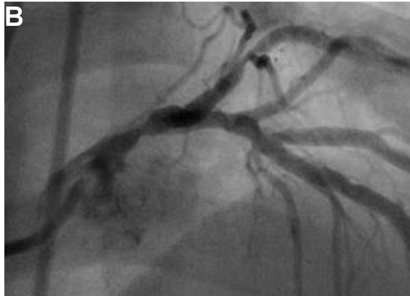
Figure 6. Clinical utility of blood flow quantification. In this example, from 81-y-old man with hypertension and dyslipidemia, relative MPI (A) with ^{82}\text{Rb} PET demonstrated only mild, reversible perfusion abnormality involving distribution of left anterior descending coronary artery. However, MFR was severely reduced globally at 1.11. Nearly entire heart had severely reduced MFR except for inferior and inferolateral walls, where it was only moderately reduced. Coronary angiography (B) showed severe stenosis of mid portion of left main coronary artery.
