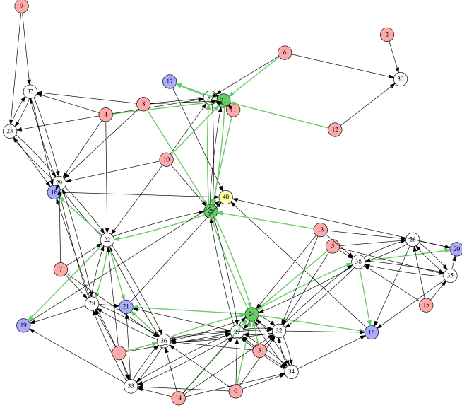
Fig. 2: An example nK scenario., with K = 12 , for the same network as in Figure 1. Sensor nodes are shown in red, aggregator nodes in white, and actuator nodes in blue. The central server, shown in yellow, is not used for the nK case. Transit nodes and links belonging to the minimum-energy aggregation and dissemination subgraph are highlighted in green.
