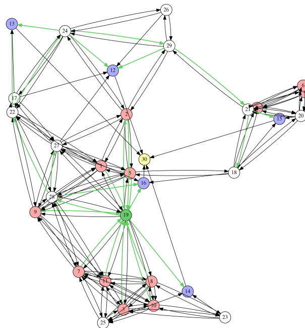
Fig. 8: An example routing solution for nK with 30 nodes. Used links and aggregating nodes are shown in green.
