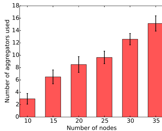
Fig. 16: Mean number of aggregating nodes used for the nK case with min-max energy optimisation, with 95% confidence intervals.
