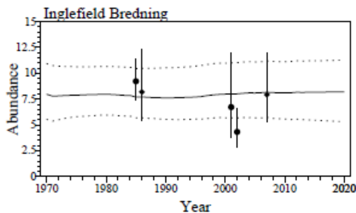
Figure 4. The trajectories of the Inglefield Breeding stock. Points with bars are the abundance estimates (given in thousands) with 90% confidence intervals. Solid curves indicate the median, and dotted curves the 90% CI, of the estimated model (Witting 2016).
