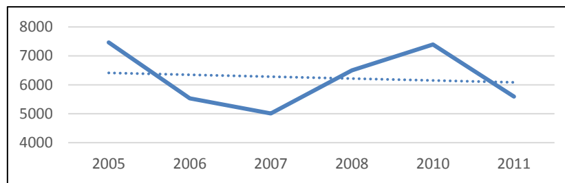
Figure 4. Summer abundance estimates of belugas in the White Sea.
