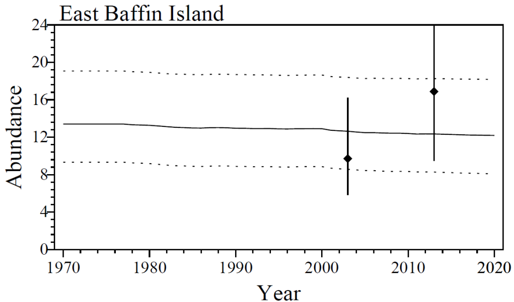
Figure 3. Population trajectory for the East Baffin Island stock. The points represent the abundance estimates (given in thousands) with 90% confidence intervals. Solid curves indicate the median, and dotted curves the 90% confidence interval for the estimated model (Witting 2016).
