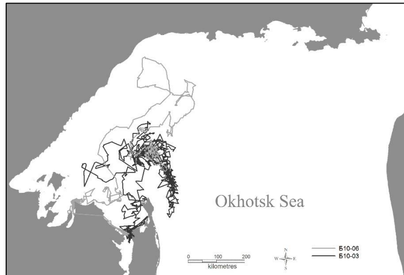
Figure 2. Satellite tracking of belugas from Sakhalin-Amur summer aggregation, 2009 (“B09” whales) and 2010 (“B10” whales). 1. Tracks of belugas, which migrated to “eastern” winter grounds. 2. Tracks of belugas, which migrated to “western” winter grounds (Shpak et al. 2012).
