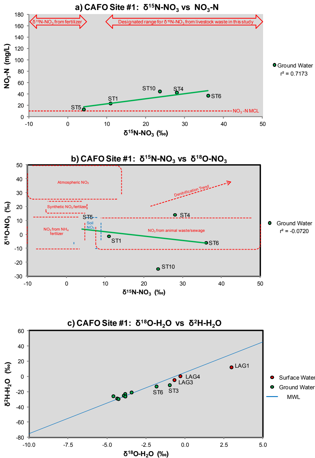
Figure 2. CAFO Site #1 isotope data relationships. Selected sample locations are identified. Green trend lines are linear correlations. The red dashed line shown in (a) is the MCL for \text{NO}_3\text{-N} . The ranges shown in (b) are adapted from Silva et al. (2002b) and Kendall et al. (2008). The MWL shown in (c) is the meteoric water line as described by Taylor (1974).
