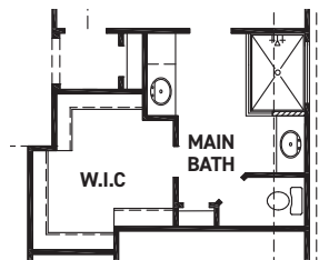
OPT. ENLARGED MAIN SHOWER
