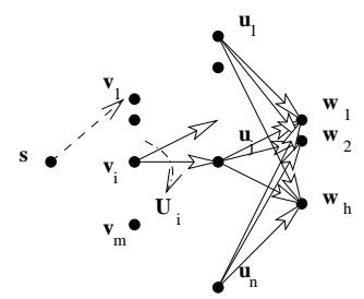
Fig. 15. Reduction from MAX-UNIQUES( k ) to Max-Sum.
