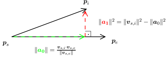
Fig. 4.8: Orthogonal projection \mathbf{a}_0 of \mathbf{v}_{s,i} on \mathbf{v}_{s,e} and rejection \mathbf{a}_1 of \mathbf{v}_{s,i} from \mathbf{v}_{s,e} .
