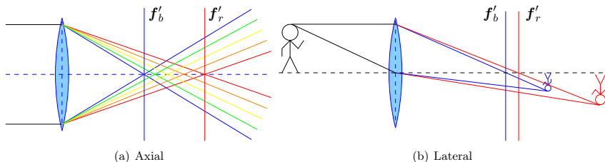
Fig. 2.17: Chromatic aberration. Reproduced based on [98]
