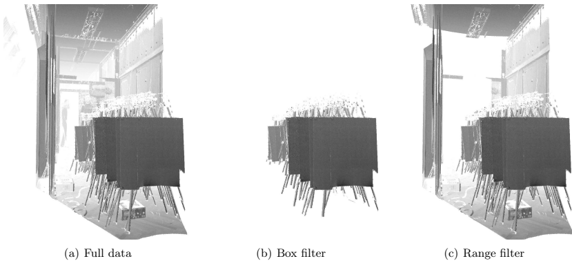
Fig. 7.8: The 55 calibration patterns from the ZAGREB data set. (a) The complete data set; (b) the data cropped with a box filter of 450 \times 130 \times 147 cm to remove everything except the calibration patterns; (c) the data cropped at a range of 5 m.
