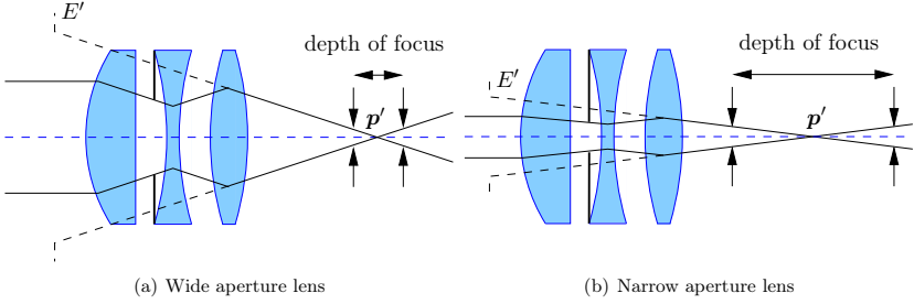
Fig. 2.14: Depth of focus with different apertures. Reproduced based on [78].
