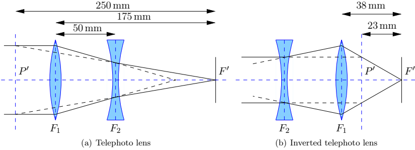
Fig. 2.13: Telephoto lenses. Reproduced based on [78].
