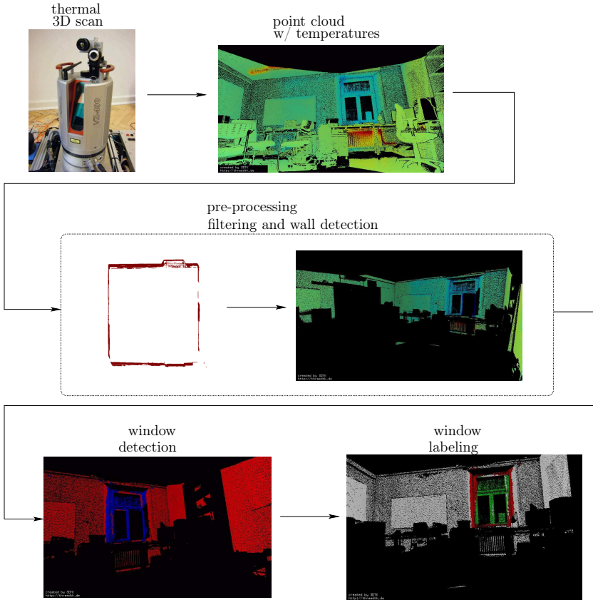
Fig. 8.14: Overview of window detection and labeling pipeline.
