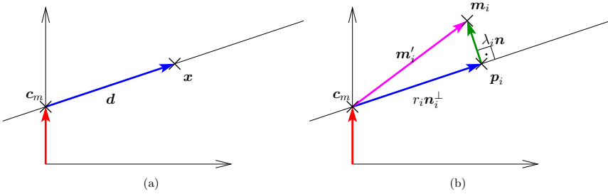
Fig. 4.14: From line equation (a) to distance to the plane (b).
