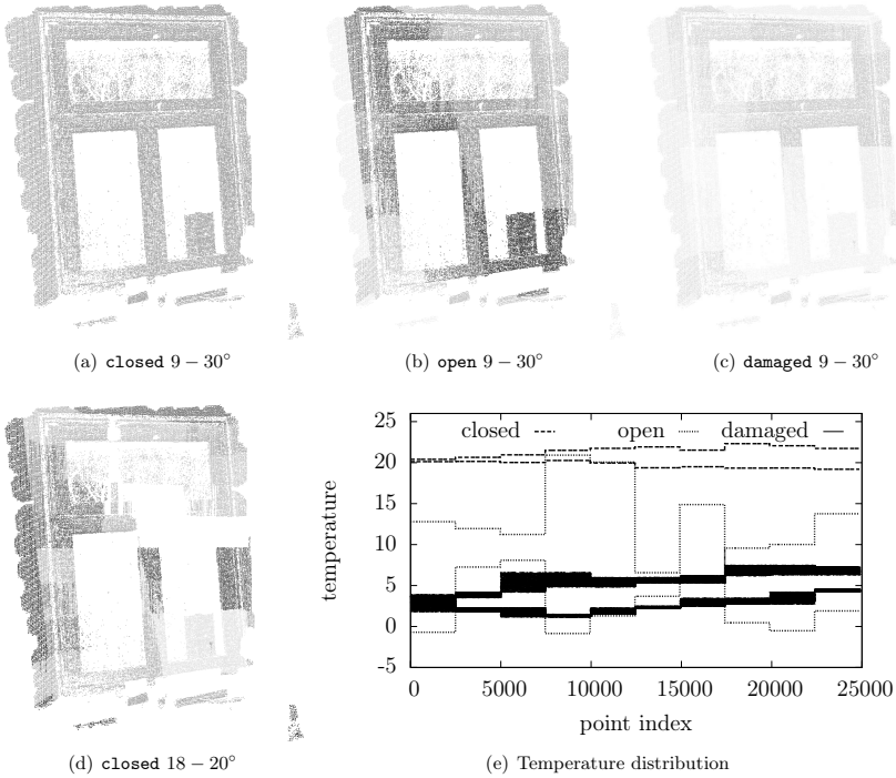
Fig. 8.21: Examples of the randomly generated temperature distributions for the labels closed , open and damaged . (a) to (d) show the window with points colored in gray scale according to the temperature. The characteristics modeled into the probability distribution functions are clearly visible. The open window has a large variance compared to the closed and damaged window. The spatial clusters, i.e., octree voxels show up as squares of the same temperature. (e) shows exemplary temperature distributions for each label. This plot points out the identical temperatures within a cluster for the open and closed window and the uniformly distributed temperature values within a cluster of the damaged window.
