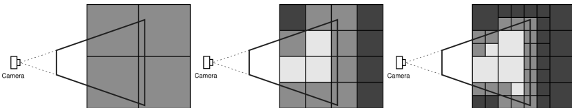
Fig. 4.6: Principle of recursive frustum culling. On each level of the octree it is decided if nodes lie completely inside (light gray), partially inside (gray), or completely outside of (dark gray) the frustum. Only for the nodes that are partially inside the frustum the culling is continued. (Source: [69])
