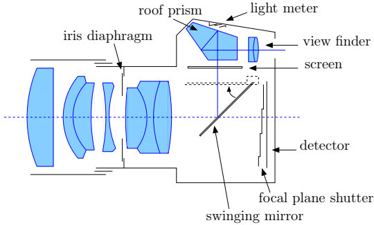
Fig. 2.11: Sketch of a lens system in a DSLR camera. Reproduced based on [78].
