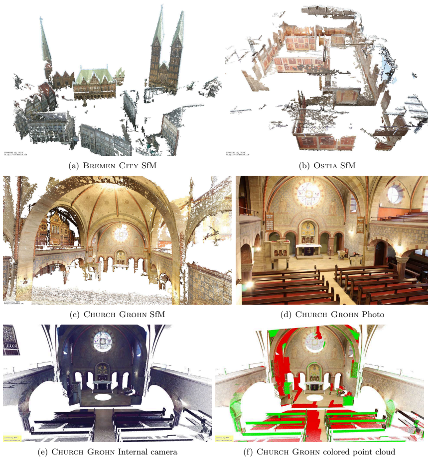
Fig. 8.36: Point clouds created with the (a) Bundler and (b)+(c) VisualSfM software. (d) A photo from the CHURCH GROHN data set. (e) First scan colored with the internal camera. (f) First scan colored with (d). Green points have normals facing away from the camera. Red points are occluded.
