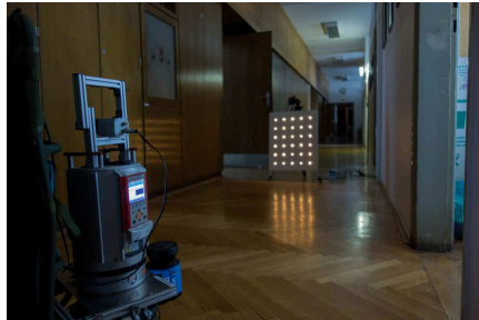
Fig. 3.1: The setup for calibration in ZAGREB.
