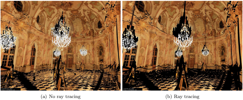
Fig. 7.23: One scan from the IMPERIAL HALL colored with the information from the photos without (a) and with (b) correction from using ray tracing. It becomes evident that the ray tracing methods removes wrongly colored points.
