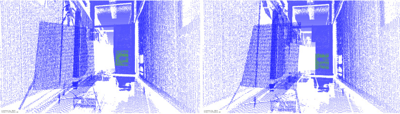
Fig. 7.9: False positives in detecting the calibration pattern. Points on the glass door are measured, leading to an additional plane.
