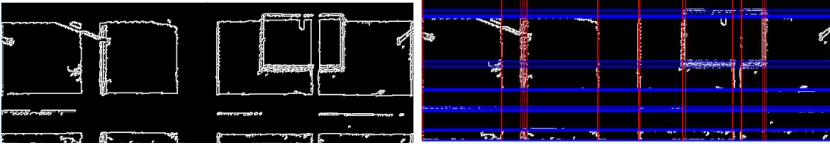
Fig. 8.6: Line detection in generated range images. Left: Image I_4 . Right: Hough lines.
