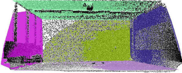
Fig. 4.20: Scan of an empty office from the AVZ data set with planes detected (RHT).
