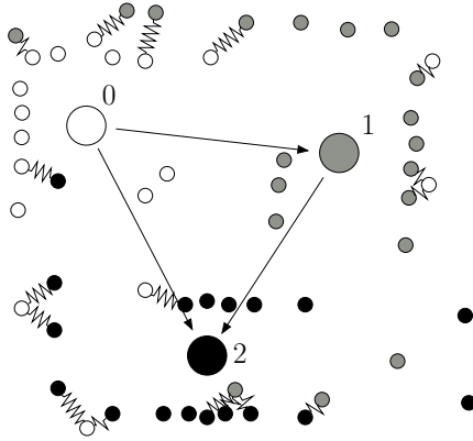
Fig. 5.4: Schematic view of the global optimization of three scans. Each scan is shown in a different gray value, the large circle represents the scan position. The correspondences resemble springs and the algorithm tries to move the scans in a way that the force on the springs is minimized. A local algorithm moves each scan individually. In the example, scan 2 would be registered to scan 1. With only few correspondences in the same area, this registration is doomed to fail. With the additional correspondences to scan 0, the chance to register the data is increased.
