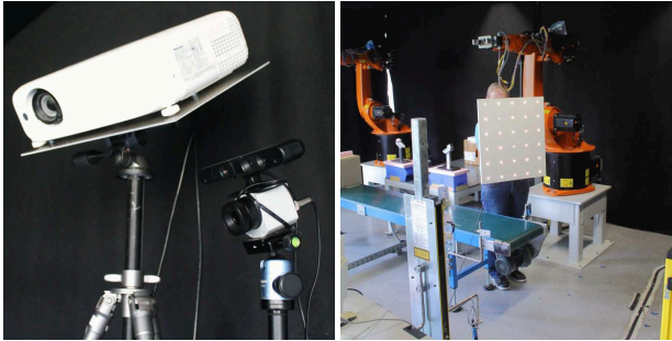
Fig. 3.10: Left: Hardware used in the experiments, a Panasonic PT-VZ575N projector, an Asus Xtion Pro live RGB-D camera and an Optris PI 400 thermal camera. Right: The calibration procedure.
