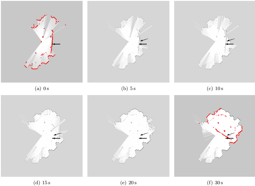
Fig. 5.2: Development of an occupancy grid map from the IMPERIAL HALL data set. The robot control loop is started and the robot stays at its starting position until t = 0 s. Then it moves until it reaches its next position at t = 25 s and stops moving again. Gray shows cells marked as unknown , white cells are empty and black cells occupied . In (a) and (f) the laser scan is depicted in red. The scanner is mounted slightly tilted downwards on the robot. Thus it sees the floor in front of it, as marked with the arrows. During the update, the wrong lines disappear.
