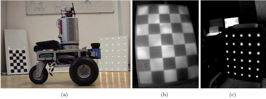
Fig. 7.1: (a) The robot Irma3D in front of two calibration patterns. (b) A chessboard pattern and (c) a light bulb pattern as seen in the thermal image.
