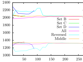
(b) Principal point c_x (solid), c_y (dashed)
