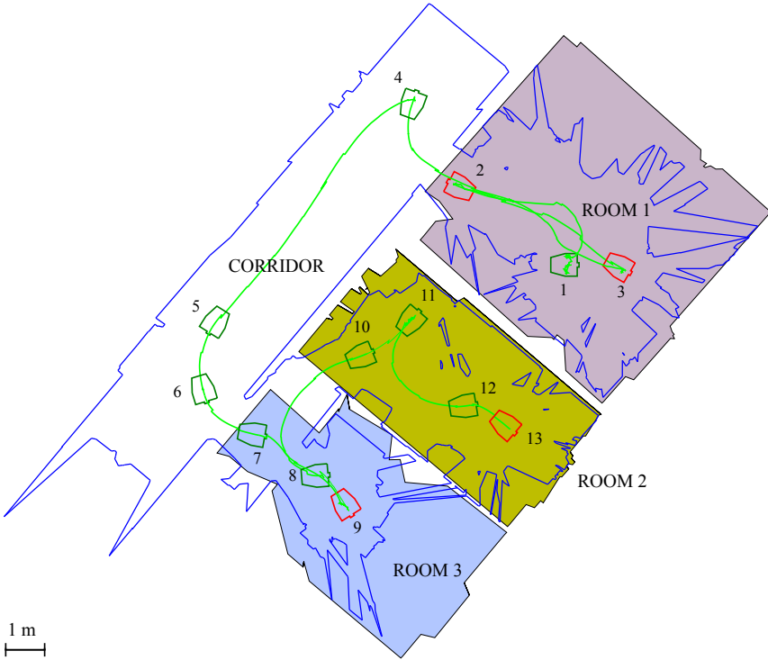
Fig. 6.4: Robot path and scanning positions during exploration.
