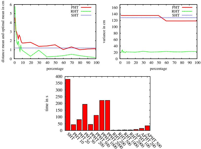
Fig. 4.21: Above: Comparison of the different point selection strategies. For the SHT all points are used and transformed into Hough Space. For the PHT only x\% of the points are chosen and the HT applied to them. For the RHT x\% times three points are chosen and the cell that corresponds to the plane spanned by these three points is accumulated. Plotted are the mean and the variance of one face of the resulting accumulator space. Below: Comparison of the runtime for the different Hough methods.
