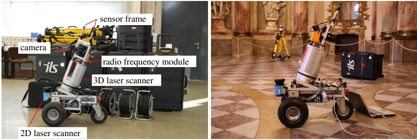
Fig. 3.5: Irma3D. Left: With the setup used in the Residence. Right: In the Imperial Hall during calibration. In the background is one of the transmitters for the iSpace localization system and a box with two reflective markers for the calibration procedure.
