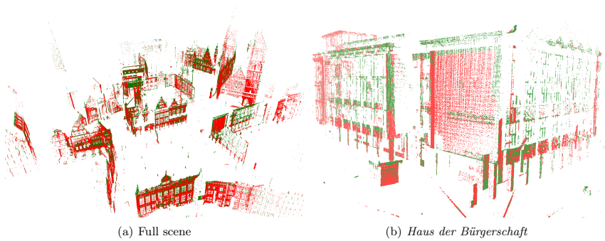
Fig. 7.26: Points with neighbors at a distance of 1 cm from the BREMEN CITY data set. Points with a temperature deviation of > 1 K are marked in green.
