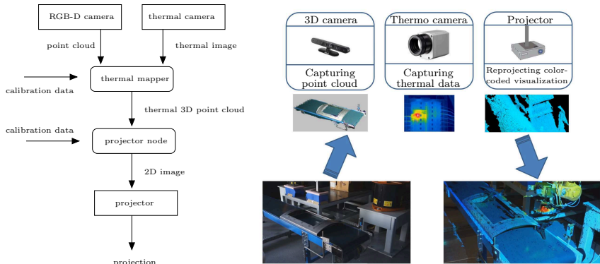
Fig. 8.24: Data flow diagram of the system.
