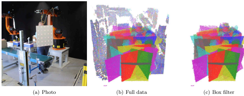
Fig. 7.13: Calibration pattern detection for the PROJECTOR data set. (a) A photo of the scene, (b) the full data set and (c) the data cropped with a box of 135 \times 130 \times 250 cm.
