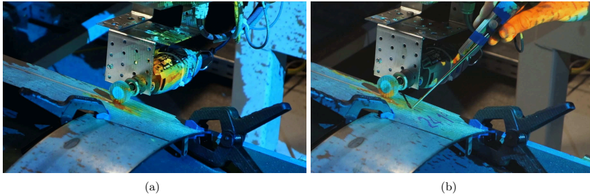
Fig. 8.26: (a) Display of temperatures during processing; the heat developing on the surface due to the grinding, as well as in the motor of the tool becomes clearly visible. (b) Measurement of surface temperature of the metal workpiece shortly after processing, using a tracked probe to specify the measurement point.
