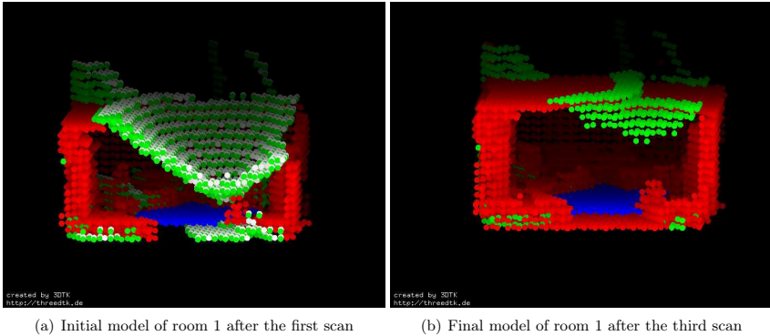
Fig. 6.6: 3D voxel based models of room 1. occupied voxels are colored red, potential position voxels (PP) are colored blue, unseen voxels are colored green. White voxels are unseen voxels that can be seen from at least one PP position in the workspace.
