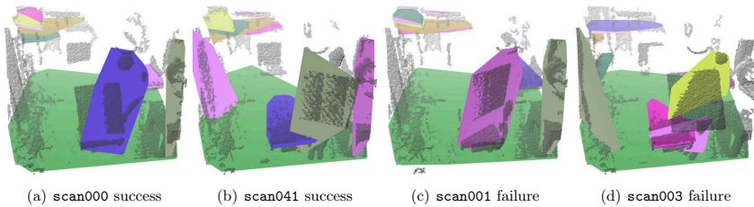
Fig. 7.14: Plane detection using the RHT in the PROJECTOR data set. The clutter in the noise leads to many false detections. The examples show that the correct detection of the plane does not determine the success of the calibration pattern detection as in one of the success cases (b) and in one of the failure cases (c) the found plane is aligned with the calibration board while in the other success case (a) and the other failure case (d) the plane intersects with the board instead.
