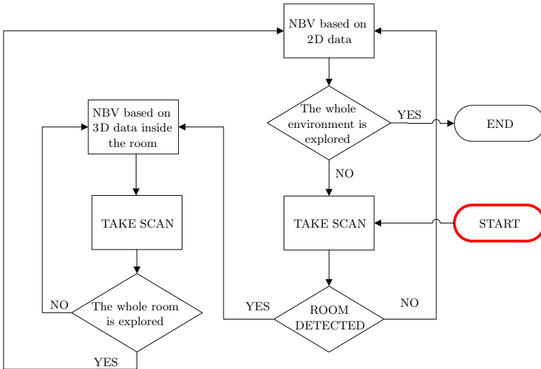
Fig. 6.1: Block scheme of the sensor placement planning algorithm
