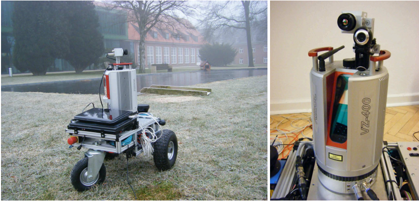
Fig. 3.2: The robot Irma3D on the Campus of Jacobs University Bremen, Germany (left). The laser scanner with the thermal camera and the webcam mounted on top (right).
