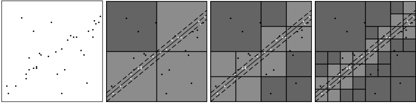
Fig. 4.17: Illustration of the speedup achieved by using an octree. Only the points in the light gray voxels are checked in the verification step. The dark gray voxels do not intersect with the line that is enlarged by a threshold. Therefore all points in these voxels are not considered in the verification step. (Source [69])
