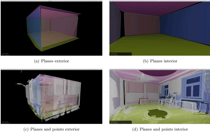
Fig. 8.12: Detected planes in the seminar room (above) and as overlay to the 3D point cloud (below).
