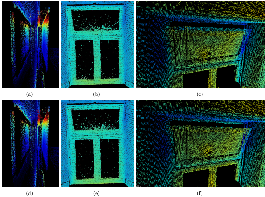
Fig. 7.20: Comparison of calibration using the second data set. Above: projection using transformation with highest reprojection error. Below: using transformation with lowest reprojection error.
