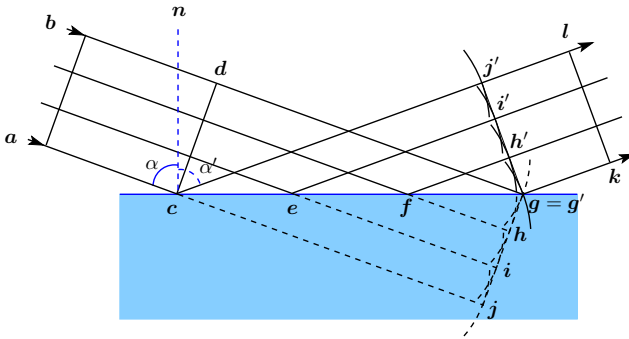
Fig. 2.5: Reflection of parallel rays on a plane surface. Reproduced based on [78].
