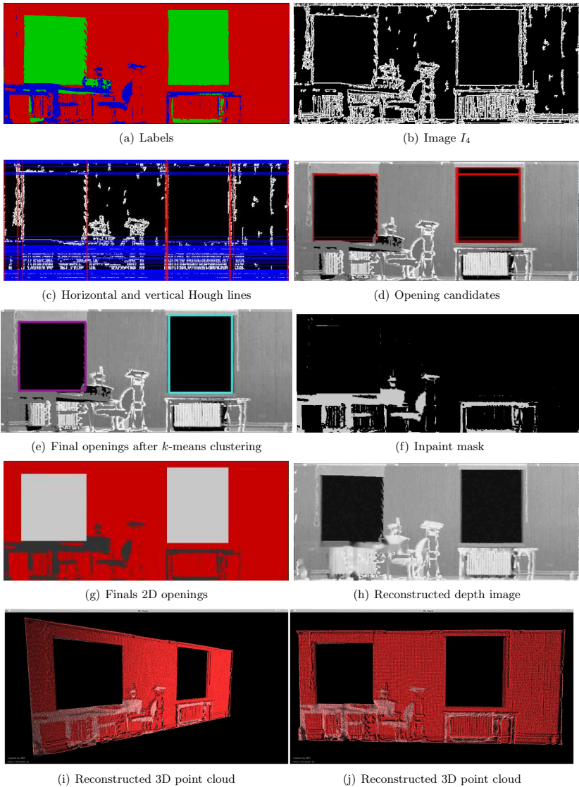
Fig. 8.13: The image processing pipeline for the surface from the seminar room containing two windows yields the reconstructed 3D point cloud of the wall.
