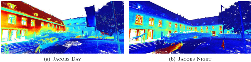
Fig. 7.28: 3D thermal model of building from the JACOBS data set highlighting the effect of diffuse sunlight on thermal measurements.
