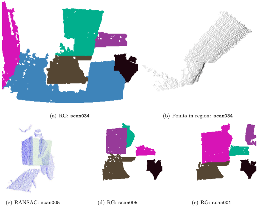
Fig. 7.16: For scan034 the RG approach fails because the coplanarity of the points not belonging to the board (b) leads to a planar patch that is larger than 1250 pixels and is thus filtered out (a). (c) shows a failure of the pattern detection with RANSAC while (d) and (e) show two successful cases for RG.
