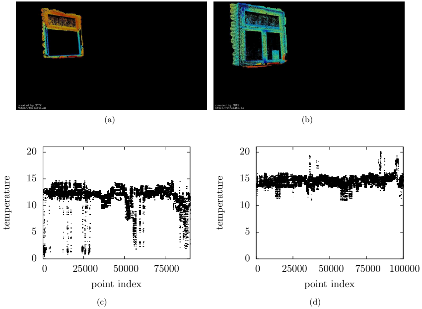
Fig. 8.19: (a) Open window colored according to the thermal distribution. (b) Closed window colored according to the thermal distribution. (c)+(d): the temperature distribution of each window, respectively.
