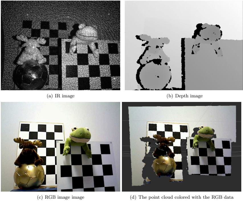
Fig. 2.32: A scene captured with the Asus Xtion Pro Live RGB-D camera.
