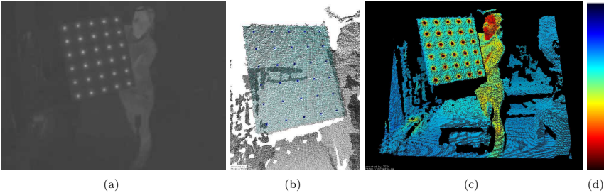
Fig. 8.25: The generation of the thermal point cloud. (a) Thermal image in gray scale (white \hat{=} 0°C, black \hat{=} 100°C). (b) The calibration procedure. The model (cyan) is fitted to the data to determine the position of the light bulbs (blue). (c) The points are colored based on the scale from 10°C to 40°C shown in (d).
