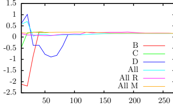
(f) Distortion coefficient k_2
