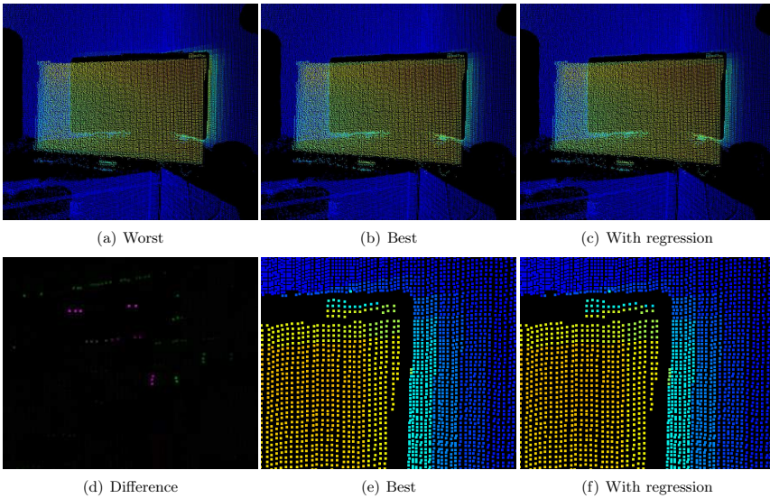
Fig. 7.19: Comparison of calibration using the first data set. Above: a computer monitor in the lab. Below: zoomed in to the top right corner of the monitor.
