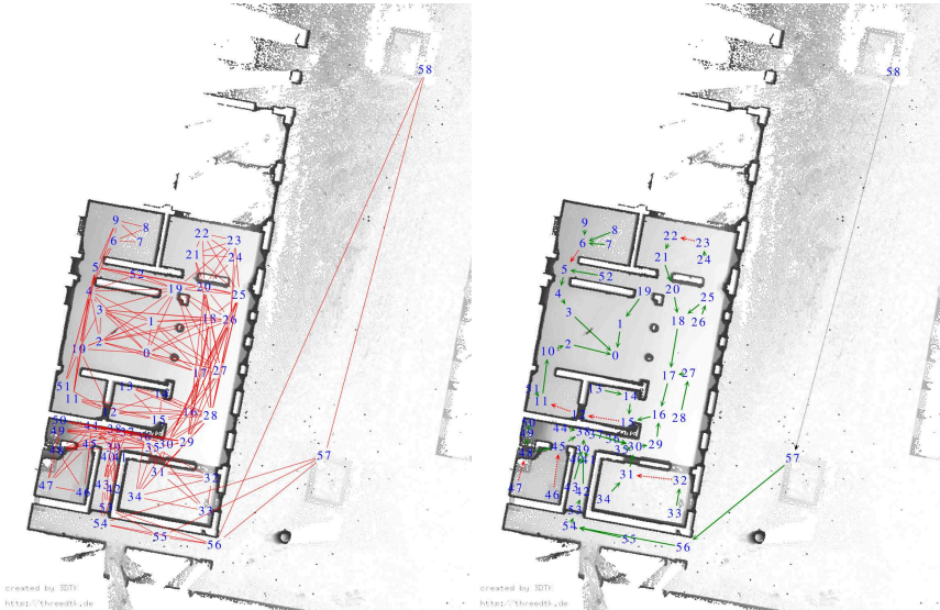
Fig. 5.7: Floor plan of the garden house in Ostia Antica generated as an orthogonal projection of the 3D model without the protection roof. The scan positions are marked. Left: The red lines show the graph used during the global optimization of the model reconstruction. Right: The arrows indicate how the scans were registered with the feature-based registration. Green arrows with solid lines indicate the scans that were registered with the standard settings. Red dashed lines mark those pairs where a modification of the parameters was necessary. The outdoor scan pair connected with a black dotted line was not registrable at all.
