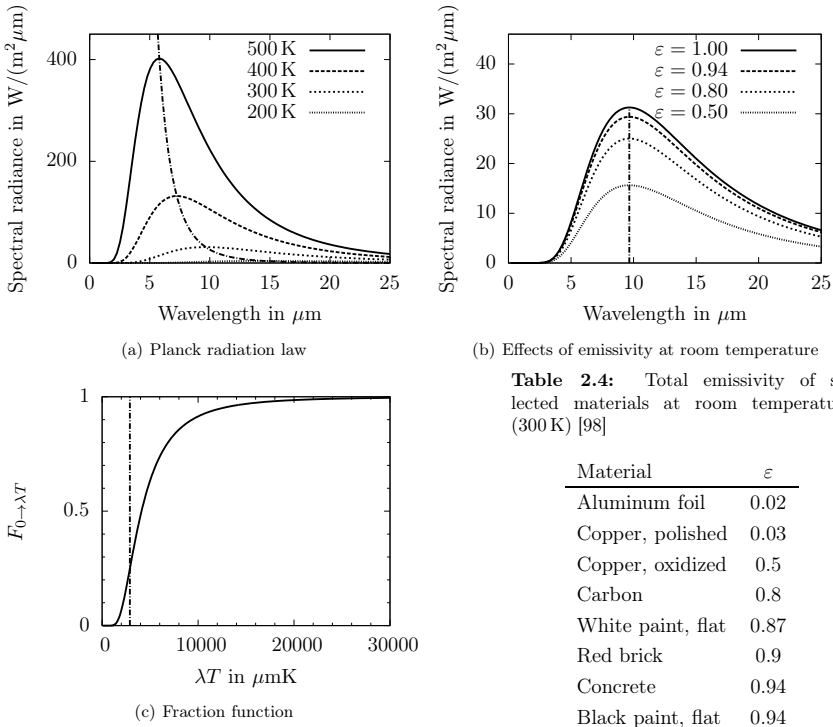
Fig. 2.22: (a) Spectral radiance for a black body based on the Planck radiation law. (b) Spectral radiance for varying emission values. (c) The fraction function plotted as a finite series explained in [187].
