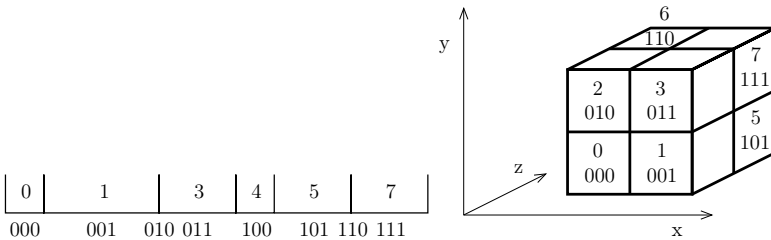
Fig. 4.3: For easy access the nodes are indexed and the points are stored consecutively. Empty voxels (index 2 and 6 in the example) have the same end pointer as their predecessors.
