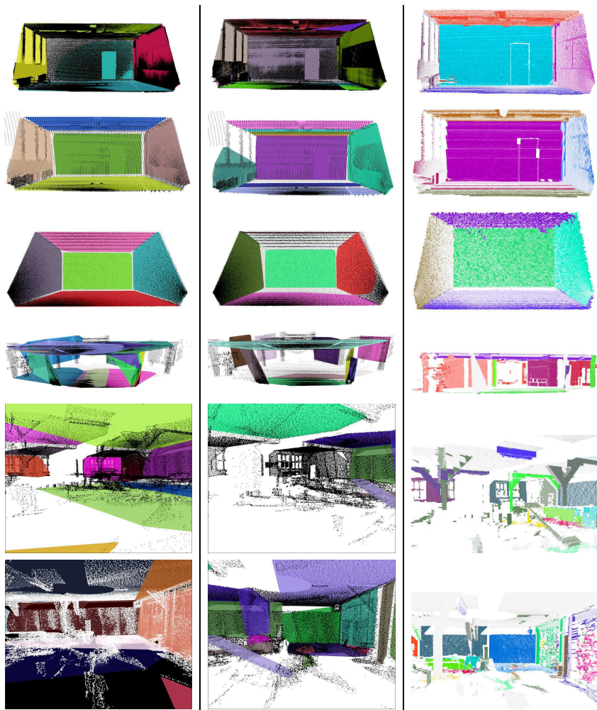
Fig. 4.23: Left: Results with the RHT. Middle: Region growing. Right: Hierarchical primitive fitting. From top to bottom: 1. AVZ data set empty room (high resolution) 2. AVZ data set empty room (low resolution) 3. simulated scan, 4. hall, 5.+6. ARENA data set
