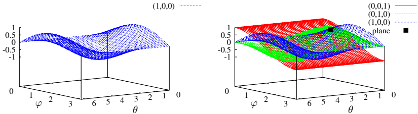
Fig. 4.18: Transformation of three points from \mathbb{R}^3 to Hough space (\theta, \varphi, \rho) . The intersection of the curves (marked in black) depicts the plane spanned by the three points.
