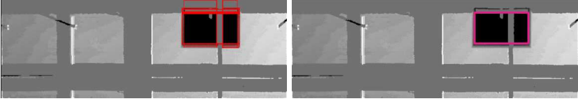
Fig. 8.7: Left: SVM learner applied to the Hough lines as presented in Fig. 8.6. Right: Result of k -means clustering and check for overlapping candidates.
