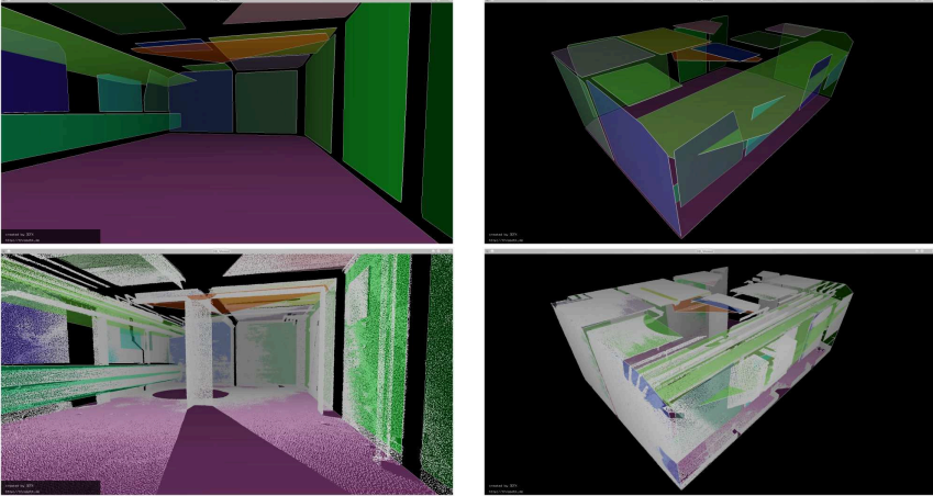
Fig. 8.2: Plane detection in the fragmented basement room. Above: Detected planes. Below: Planes and 3D points.
