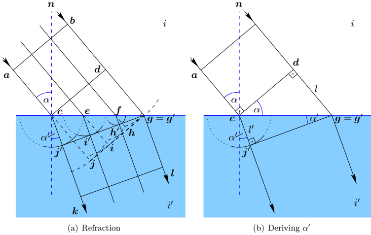
Fig. 2.6: Refraction on a plane surface. (a) Reproduced based on [78].
