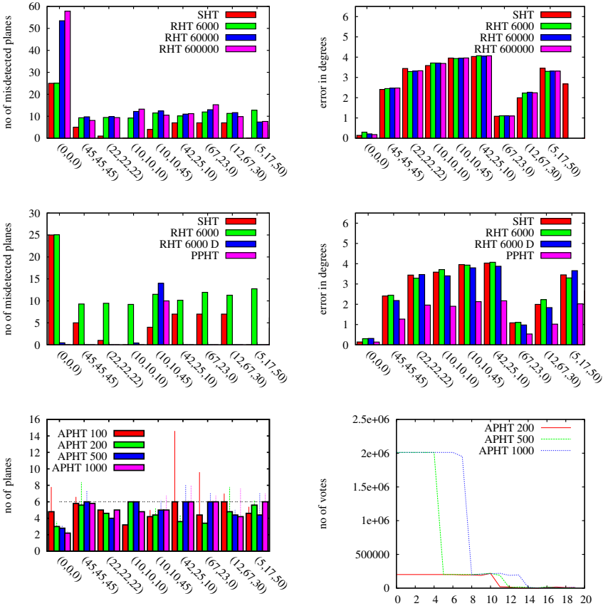
Fig. 4.22: The experiments were carried out on the modeled cube scan rotated by (\alpha_x, \alpha_y, \alpha_z) without plane fitting after the HT. Above: Comparison of the RHT with the SHT when applying it on the test cube. For RHT x , x triples of points are selected. Center: Comparison of different Hough methods with respect to their ability to correctly detect all planes in a data set and their accuracy. Below: Results for running the APHT with different maximum stability counts on the cube data set.
