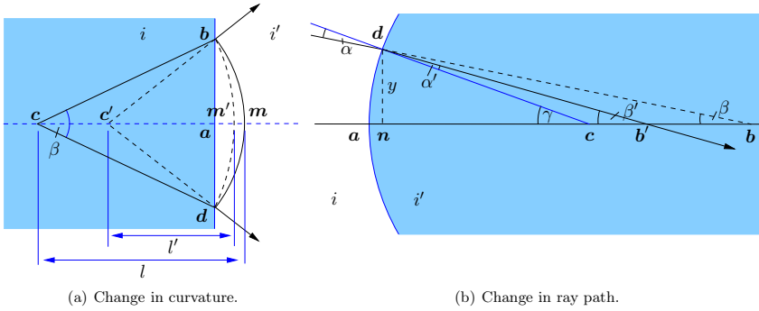
Fig. 2.7: Effects of refraction reproduced based on [78]. (a) Change in curvature at a plane surface. (b) Change in ray path at a spherical surface.
