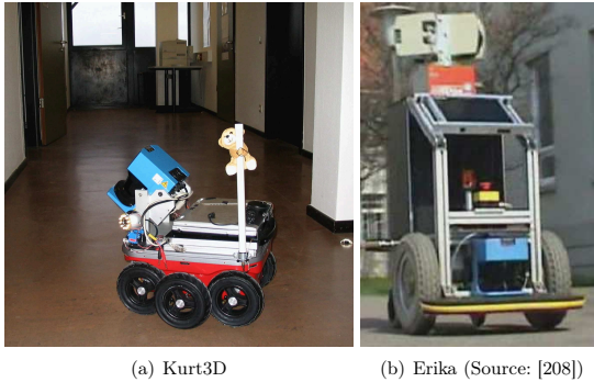
Fig. 2.3: Mobile robots with rotating 2D laser scanners.
