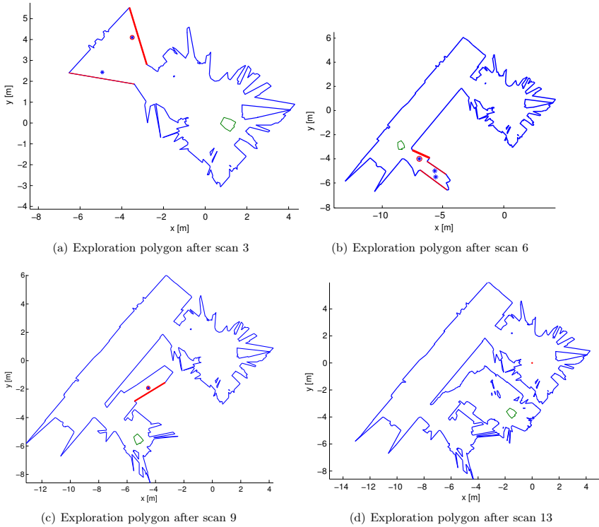
Fig. 6.5: Important exploration polygons during the experiment (jump edges are in red color and 2D NBV scanning positions marked with cross characters in red circles).
