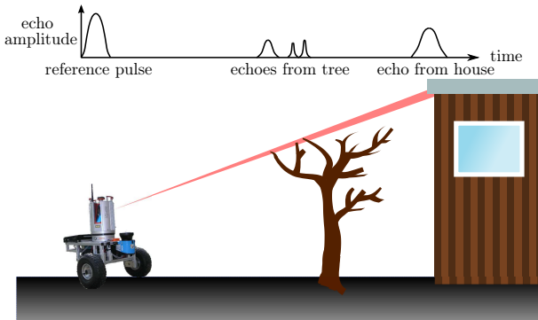
Fig. 2.25: The principle of full wave analysis. Multiple echoes are returned when the beam is split up at edges. Source: [64]
