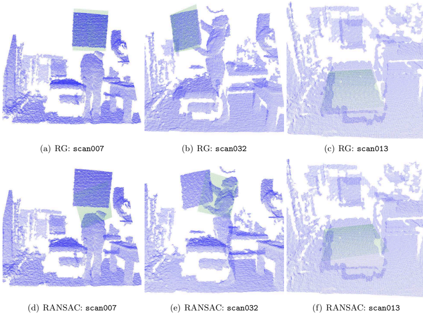
Fig. 7.15: Three failure cases in the Projector data set. In scan007 and scan032 the data is calibration pattern is cropped. In scan013 it is hardly distinguishable from the conveyor belt and the top is ragged due to the low incident angle.
