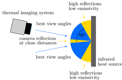
Fig. 7.24: Best view angles for thermography. Straight-on measurements on high reflective materials at close distances cause direct camera reflection, oblique angles are prone to errors due to overall reflection. Reproduced based on [74].
