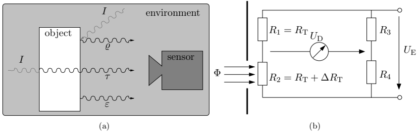
Fig. 2.23: (a) Surface radiation of an object. Reproduced based on [157]. (b) Principle of a bolometer. Reproduced based on [178].
