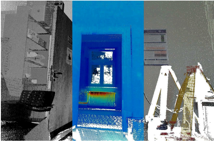
Fig. 7.27: Laser scan with reflectance (left), thermal (middle) and color (right) information.
