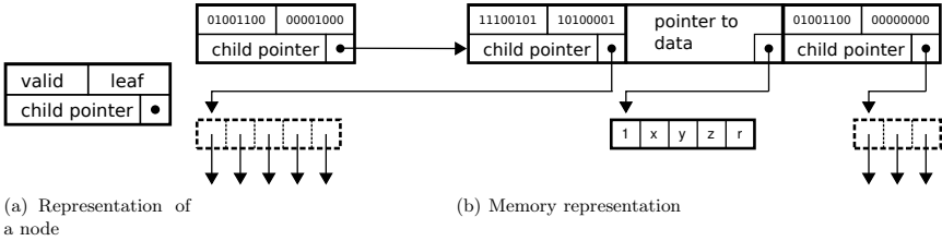
Fig. 4.2: A small example of an octree as it is stored using the proposed encoding (Source: [69]). The node in the upper left has three valid children, one of which is a leaf. Therefore, the child pointer only points to three nodes stored consecutively in memory. The leaf node in this example is just a pointer to an array which stores both the number of points and the points with all their attributes.
