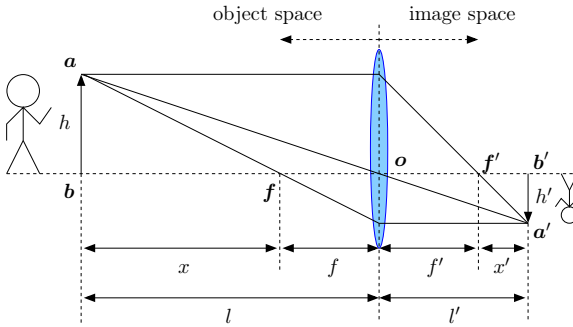
Fig. 2.9: Thin lens model. Reproduced based on [78].
