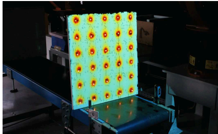
Fig. 8.27: The thermal projection of the temperature distribution of the calibration pattern for the thermal camera. It becomes clear that the area around the small light bulbs is heated up.
