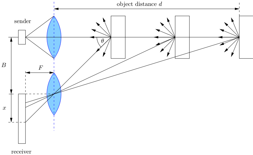
Fig. 2.27: Principle of triangulation. Reproduced based on [61].
