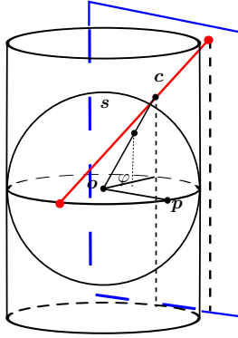
Fig. 4.11: Schematic of the construction rule for the Pannini projection. The sphere point s is first mapped onto the point c on the cylinder and then projected onto the tangent plane. This corresponds to the rectilinear projection of the cylindrical projection of the sphere. p is the point corresponding to the spherical coordinates (\theta = 0, \varphi = 0) . (Source: [107])
