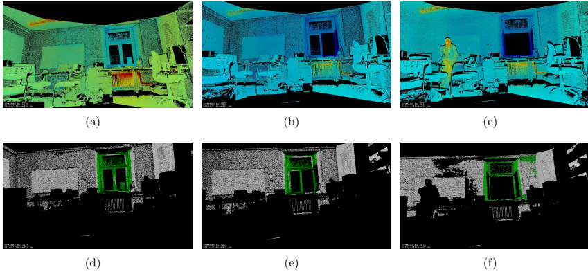
Fig. 8.22: (a)-(c): Three original thermal 3D point clouds with temperature values. (d)-(f): The detected windows under different circumstances, i.e., (d) closed, (e) semi-open, and (f) fully open are shown in green.
