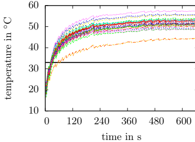
Fig. 7.3: Temperature trend of the 30 light bulbs over a period of 11 min.
