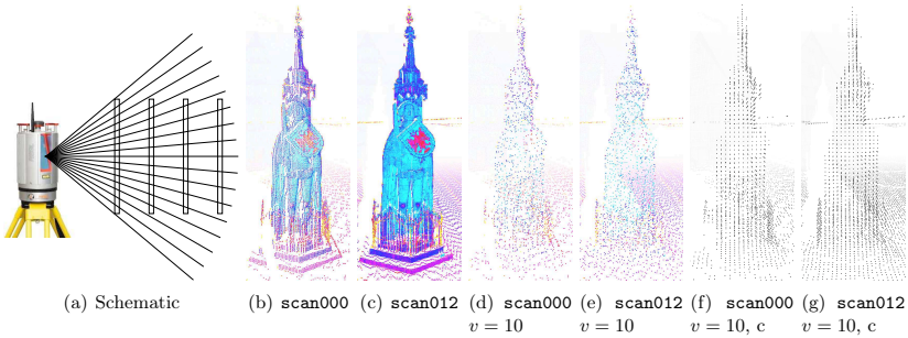
Fig. 4.4: (a) Schematic of the decreasing point cloud density based on the distance to the sensor. Due to the angular sweeping of the laser beam with increasing distance the density decreases, i.e., a wall of identical size is sampled with fewer points. (b)+(c) The Bremen Roland seen from two positions in the BREMEN CITY data set. scan000 has a distance of \approx 65 m to the statue while scan012 has a distance of \approx 33 m. (d)+(e) The scans reduced to a voxel size of 10 cm. One point per voxel is randomly chosen. (f)+(g) The center of each occupied voxel is chosen during reduction.
