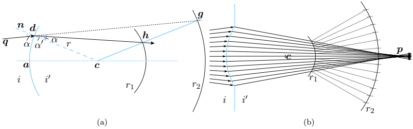
Fig. 2.8: Graphical construction of refraction on spherical surfaces reproduced based on [78]. (a) Construction of a single refracted ray. (b) Refraction of multiple rays coming from a distant point source.
