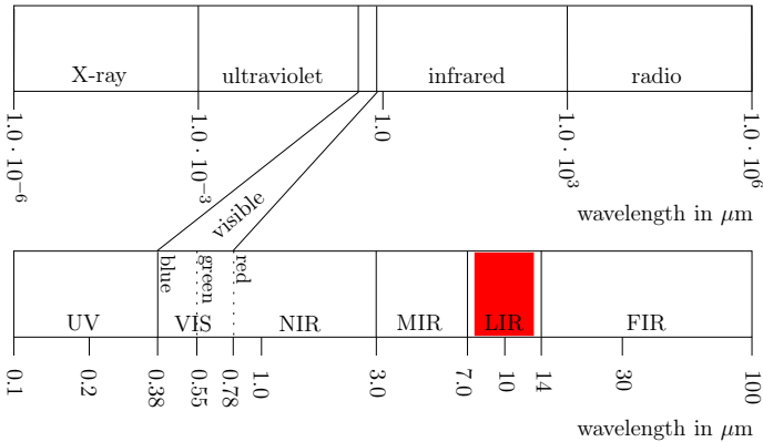
Fig. 2.20: Presentation of the infrared spectrum within the electromagnetic spectrum (reconstructed based on [178]).
