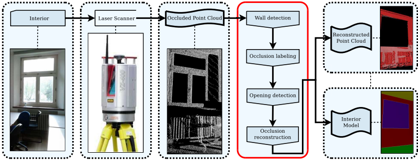
Fig. 8.1: Reconstruction pipeline.
