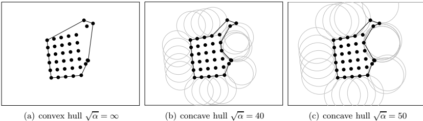
Fig. 8.3: The Alpha Shapes algorithm using varying parameters.
