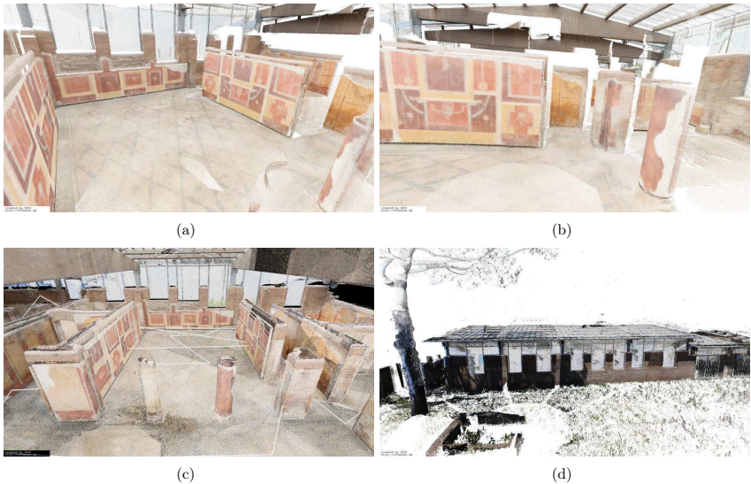
Fig. 5.8: The model of the garden house in Ostia Antica. (a) and (b) Two views of the data acquired on the first day. (c) The complete model with data from all days. The white lines mark the scanning sequence. (d) Outside view of the complete model.
