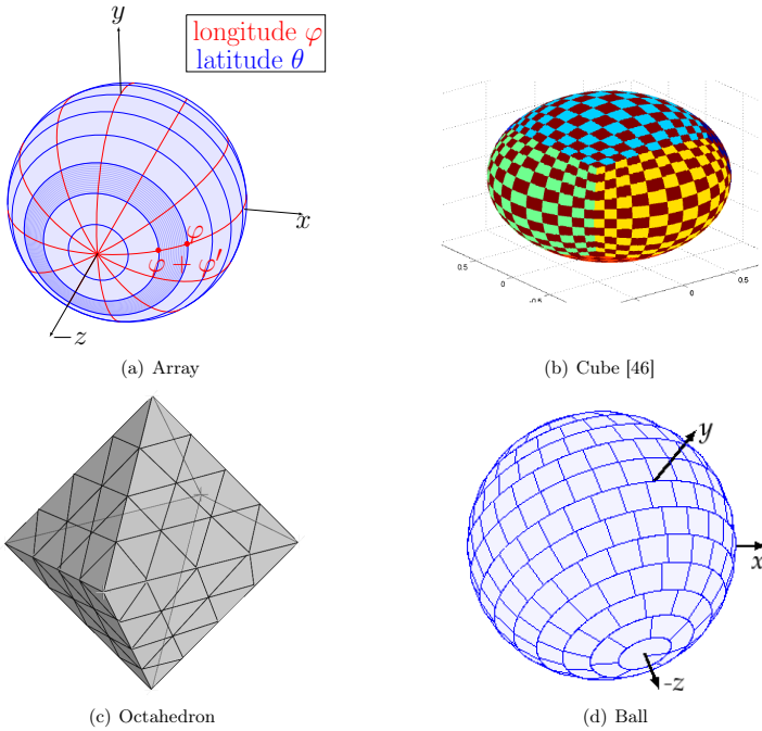
Fig. 4.19: (a) - (d): Mapping of the accumulator designs onto the unit sphere. (a) also illustrates the calculation of the length of a longitude circle at \varphi_i that determines the discretization for the ball design. The segment in question is the darker colored one.
