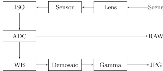
Fig. 8.30: Typical processing steps in the image formation.
