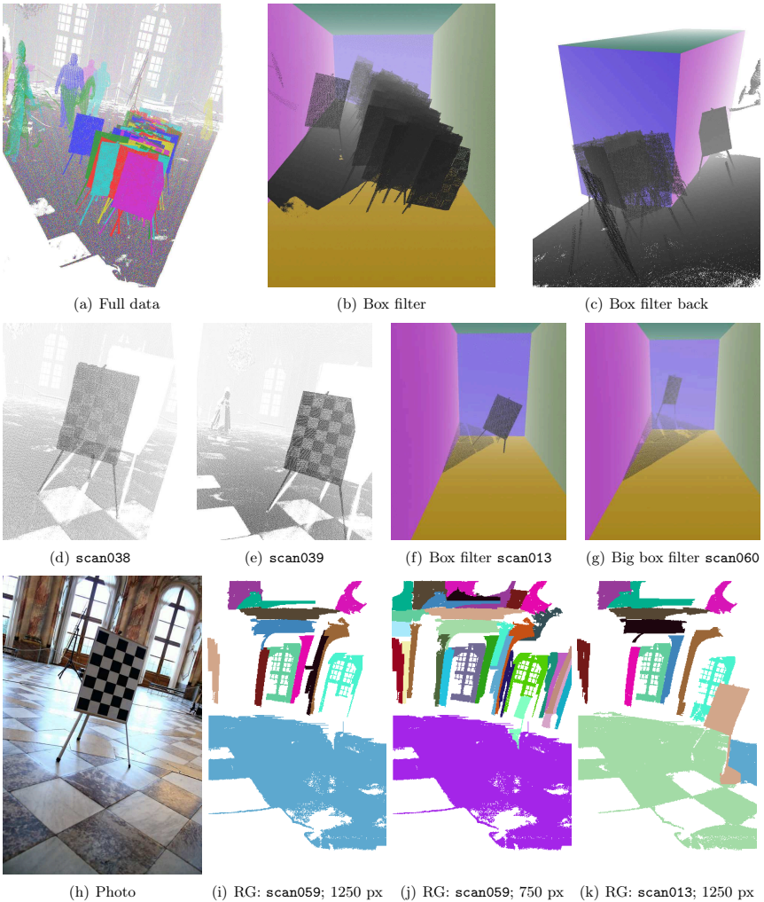
Fig. 7.12: Calibration pattern detection in the IMPERIAL HALL of the Würzburg Residence Palace. The full data set (a) and two sample scans (d) and (e). The box filter (b),(c),(f) and a slightly larger box filter (g). The planar patches found by region growing with at least N_{\min} = 1250 pixels (i) and (k) and N_{\min} = 750 pixels (j), respectively.
