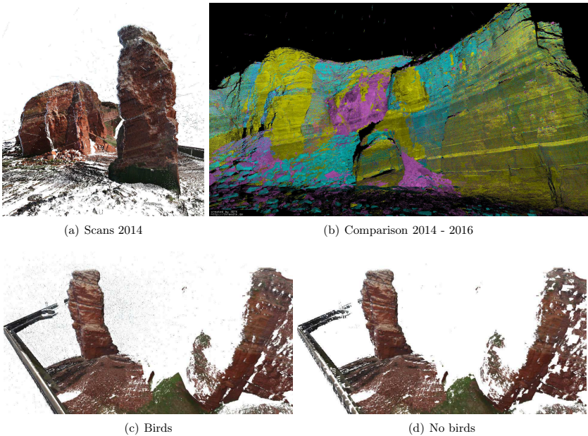
Fig. 7.31: HELGOLAND. (a) Color scans of the Lange Anna from 2014. (b) Comparison of scan position 4 from the different years. Scans are colored by reflectance information. Cyan, magenta and yellow indicate the different years. (c) Scan positions on the upper part from 2014. (d) Scan positions on the upper part from 2014 with a bird filter.
