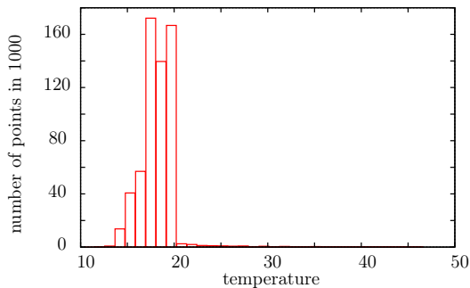
Fig. 8.17: Typical temperature distribution of a 3D scan with walls and windows only.
