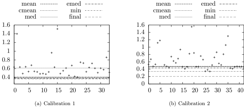
Fig. 7.18: Reprojection error for extrinsic calibration. The x -axis represents the indices of the data pairs.
