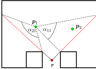
Fig. 6.2: Selection criterion based on angles of visibility.
