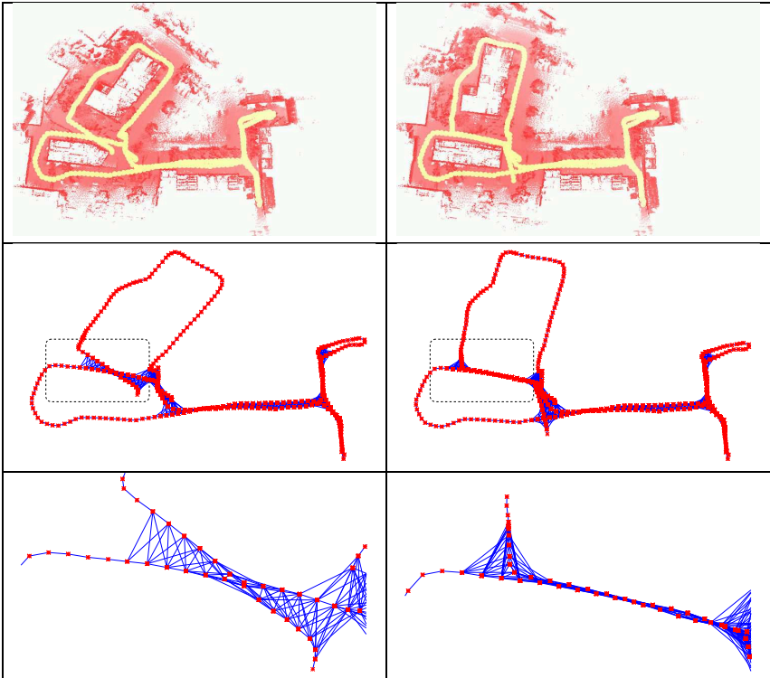
Fig. 5.6: LUM iterations before and after the fourth closed loop of the HANNOVER1 dataset. Above: Forth loop closing after 1 iteration and after 20 iterations. Middle: The corresponding graphs. Below: Zoom into the boxed areas. When turning into the upper loop, the pairwise registration fails. By loop closing and graph recomputation this failure is corrected and the robot paths are merged. The zoomed-in graph representation shows how more links are added to the graph after merging the paths partially in the first iterations. (Source: [29])
