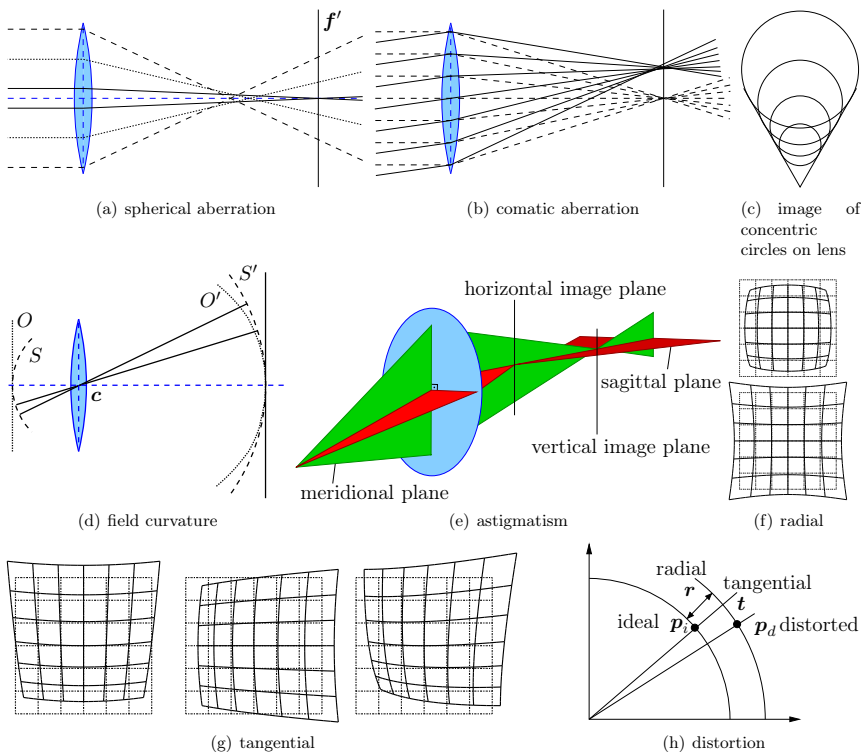
Fig. 2.16: The five primary aberrations. Reproduced based on [98] (a),(d),(f) [78] (b),(c), [143] (e) and [202] (h).
