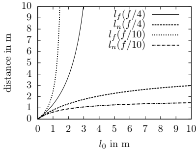
Fig. 2.19: Minimum and maximum distance for objects to cause the maximum allowed blur when focusing on l_0 using a Canon EOS 1000D camera with EF-S18-55 mm IS II lens.
