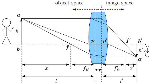
Fig. 2.10: Thick lens model. Based on [78].
