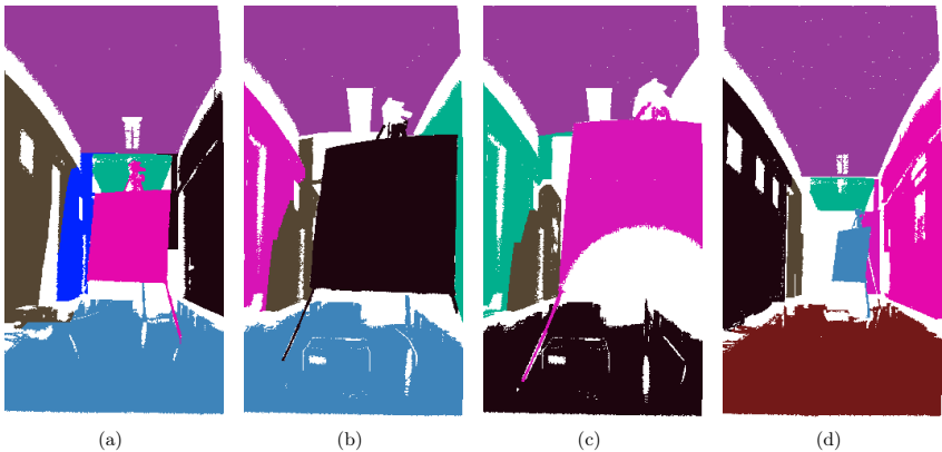
Fig. 7.11: Plane detection in range images.
