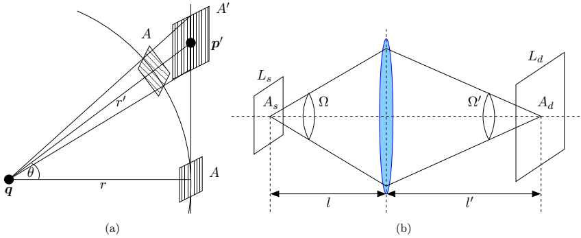
Fig. 2.18: (a) Variation of radiance for a flat surface at an incident angle \theta . (b) Lens imaging an extended source. Reproduced based on [78].
