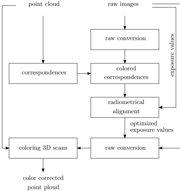
Fig. 8.31: Framework for radiometrically aligning point clouds.
