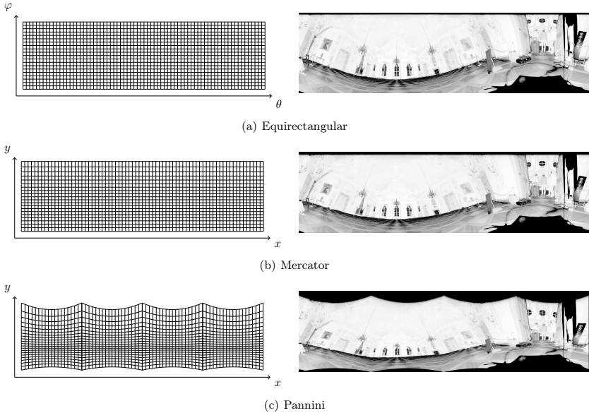
Fig. 4.10: Example of the different projection methods. On the left are the latitude and longitude lines as they appear in the projection with a resolution of 5^\circ . The field of view is 0^\circ \leq \theta \leq 360^\circ horizontally and -40^\circ \leq \varphi \leq 60^\circ vertically as for the Riegl VZ-400. On the right is the first scan from the WHITE HALL data set as panorama image. Note that the scanner was tilted for better view of the ceiling, thus the edge between wall and floor is curved in all projections.
