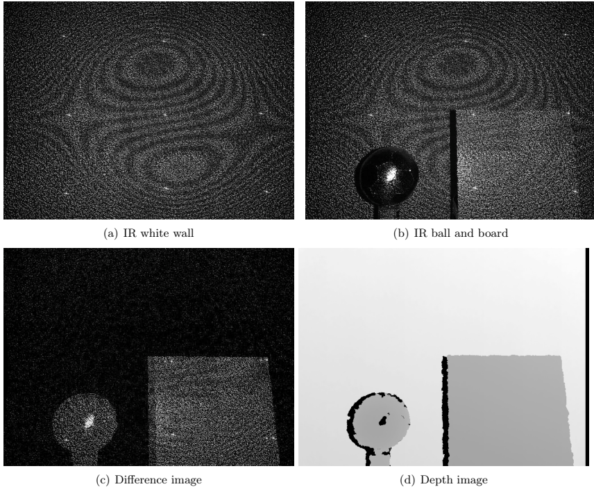
Fig. 2.31: Images taken with the Asus Xtion Pro Live RGB-D camera. (a) The infrared image captured by the infrared camera from a white wall. (b) The infrared image with a ball and a board in front of the wall. (c) The difference image between (a) and (b). (d) The depth image corresponding to (b).
