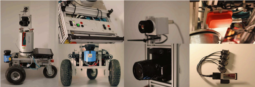
Fig. 2.2: The mobile robot Irma3D. From left to right: side view of the robot with all its sensors; Above: The control panel with switches for the two electric circuits and sockets for charging the batteries. The laptop mount fixes a laptop above the control panel. Below: Front view showing the 2D laser scanner and two small digital cameras that are attached to the robot for easier navigation; The thermal camera (above) and a DSLR camera (below) that are mounted on top of the laser scanner to sense thermal properties and color information of the environment to enhance the point clouds; Above: An IMU is mounted underneath the chassis next to the rear wheel. The position provides maximum shielding from the magnetic fields generated by the motors and the 3D laser scanner. Below: An ExpressCard to RS-232 Adapter is used to connect modern laptops without serial ports to the Volksbot motor controller and the IMU. (Source [150])
