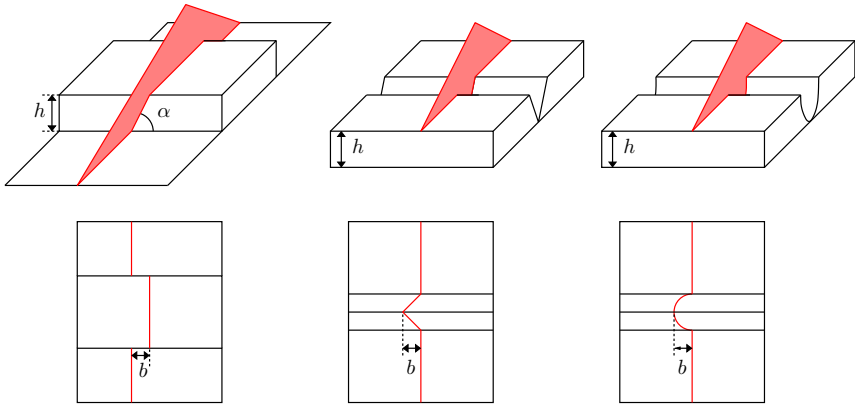
Fig. 2.28: Principle of line scanning. Reproduced based on [61].
