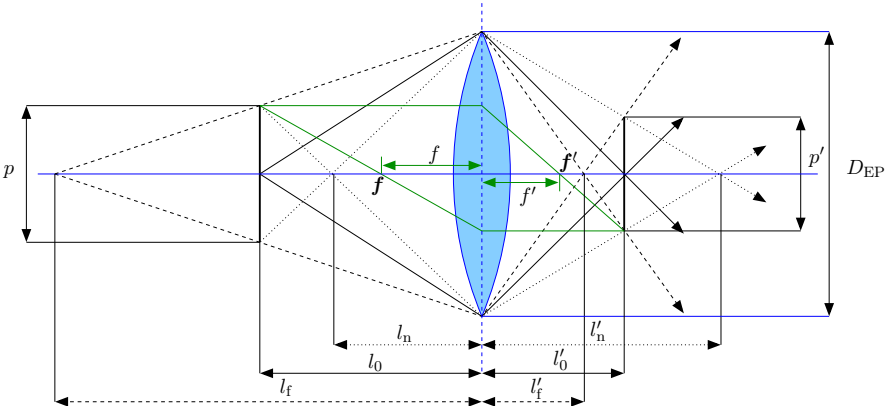
Fig. 2.15: Depth of field. Objects at a distance of l_0 are in focus, while the l_n gives the distance of the near plane and l_f the distance of the far plane the thresholds leading to the maximum allowed blur. Reproduced based on [163]. The green construction lines assert the distances of the object and image plane in focus.
