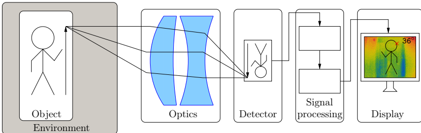
Fig. 2.21: The radiometric chain for thermal imaging.
