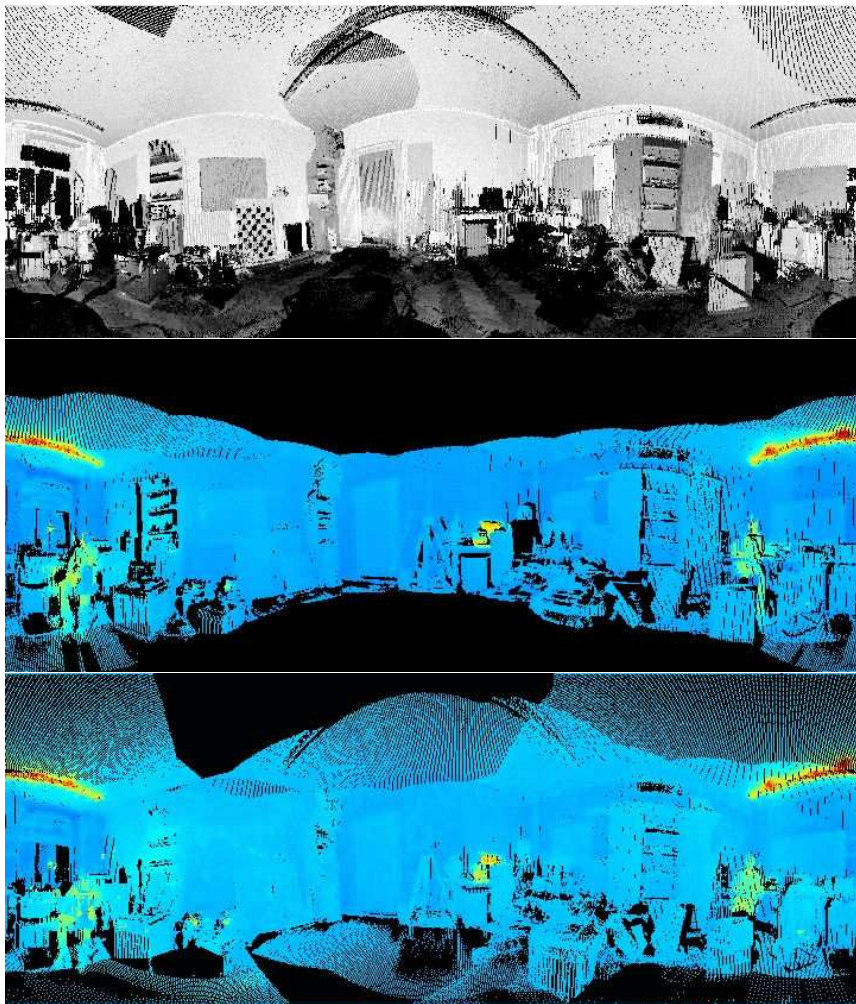
Fig. 6.8: Panorama images of room 1. Top: The entire room with reflectance values as captured by the laser scanner using 3D exploration. Middle: The part captured with thermal information using 2D exploration. Bottom: The part captured with thermal information using 3D exploration. Note that the thermal camera has a drastically reduced field of view as compared to the laser scanner.
