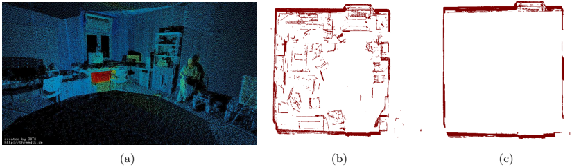
Fig. 8.16: (a) A 3D thermal model of the AUTOMATION LAB at Jacobs University Bremen. (b) 2D projection of the room with the xy -axis colored in red. (c) The detected outer rectangular shape, or walls, of the room.
