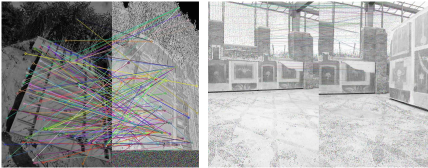
Fig. 8.34: Sift feature matching, the lines connect the best feature matches according to the descriptor matching. Left: Comparison of Sift features in the BRÄUTIGAM data set between a photo as gray-scale image and the intensity image of a laser scan. The lines connect the feature correspondences. Right: Two photos from the OSTIA data set.
