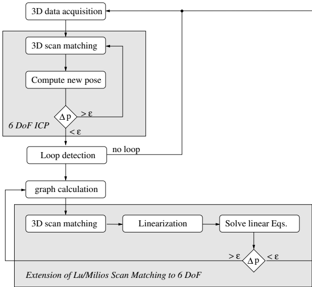
Fig. 5.5: The interaction of ICP and the global optimization in the overall algorithm. The threshold \epsilon used to determine if a scan changed its pose is the same in both algorithm parts. (Source: [29])
