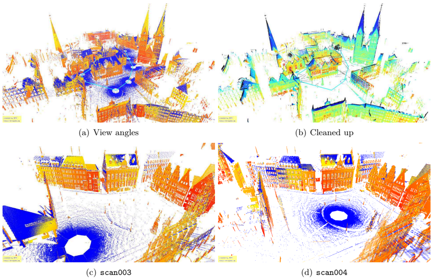
Fig. 7.25: The complete scene from the BREMEN CITY data set. (a) The points colored based on the angle between the normal and the view vector. Blue points have an angle greater than 60^\circ . (b) The scene without the points with an angle greater than 60^\circ colored based on temperature values. (c) + (d) Two scans from the Market square, showing the different view angles.
