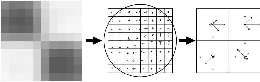
Fig. 4.13: Illustration of the creation of a Sift descriptor from a gray scale image using local image gradients. The key-point is located at the center of the patch. For clarity the alignment to the main gradient orientation has been omitted.
