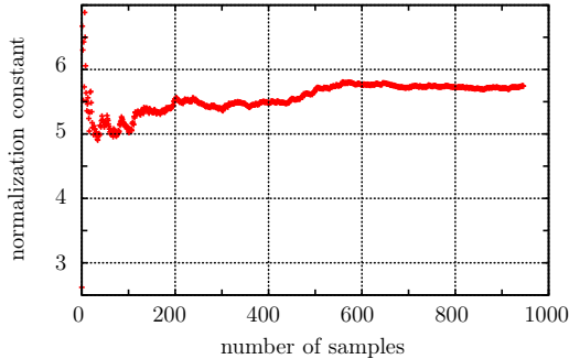
Fig. 8.23: The convergence of the mean sequence; the approximation of the normalization constant of a closed window with 1,000 samples.
