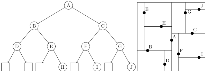
Fig. 4.7: k D-tree.
