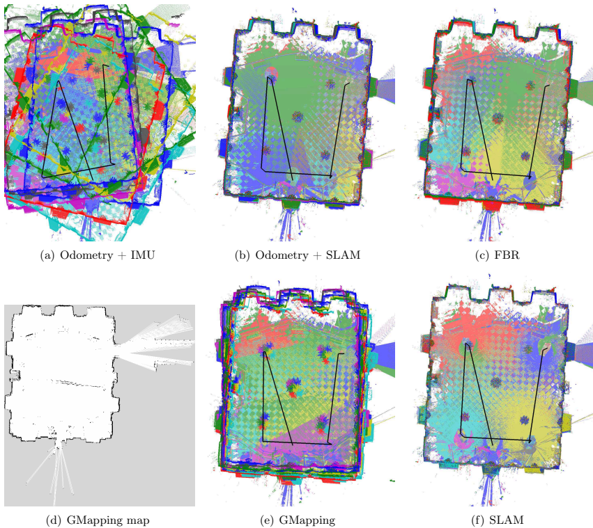
Fig. 5.9: Floor plan of the WHITE HALL. Projection of the 3D point cloud without the roof using poses from odometry and IMU (a), slam6D with pose estimates from odometry and IMU (b), feature-based registration (c), GMapping (e), slam6D with pose estimates from GMapping (f). Each scan is drawn in a different color. The black line connects the scan positions. (d) shows the map created from GMapping using the 2D laser scanner.
