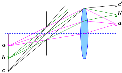
Fig. 2.12: Vignetting caused by the lens as effective field stop. Reproduced based on [78].
