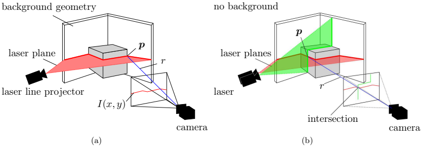
Fig. 2.29: Laser line projector systems using one (a) or two (b) laser planes.
