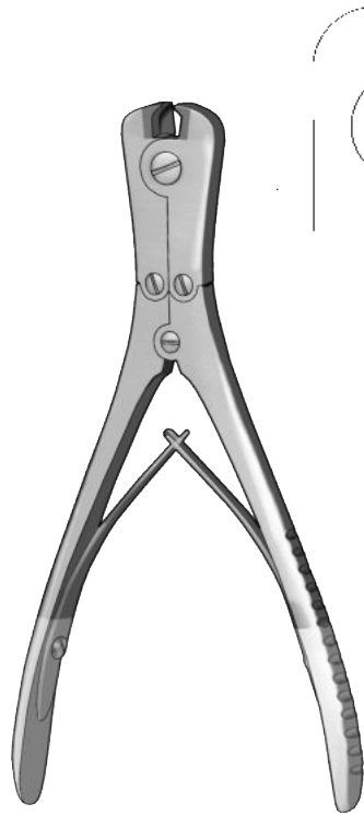
OM 46-0631 7" (178mm) front and side cutting with carbide inserts cuts up to .062" (1.6mm)
