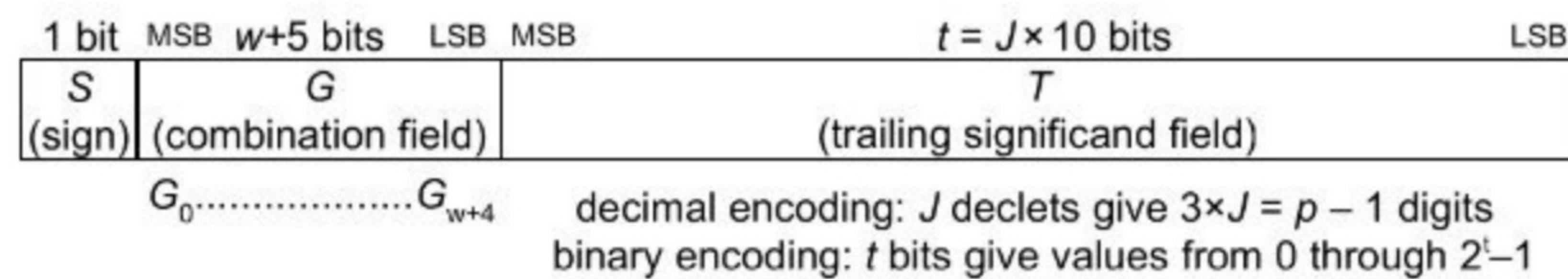
Figure 3.2—Decimal interchange floating-point formats
