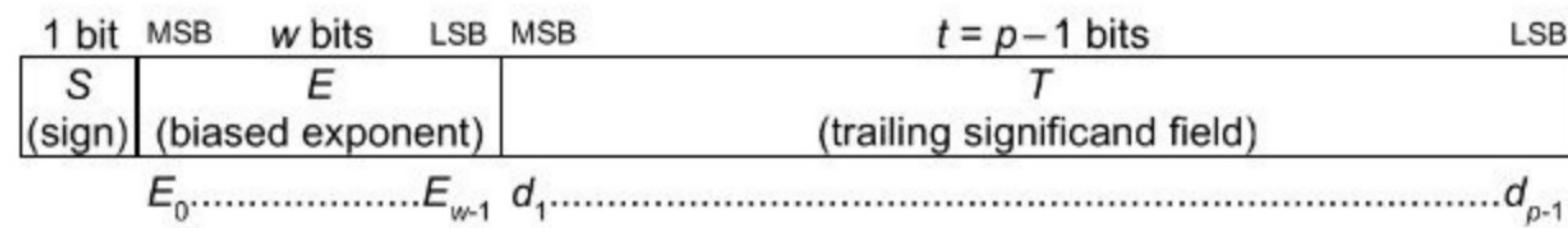
Figure 3.1—Binary interchange floating-point format
