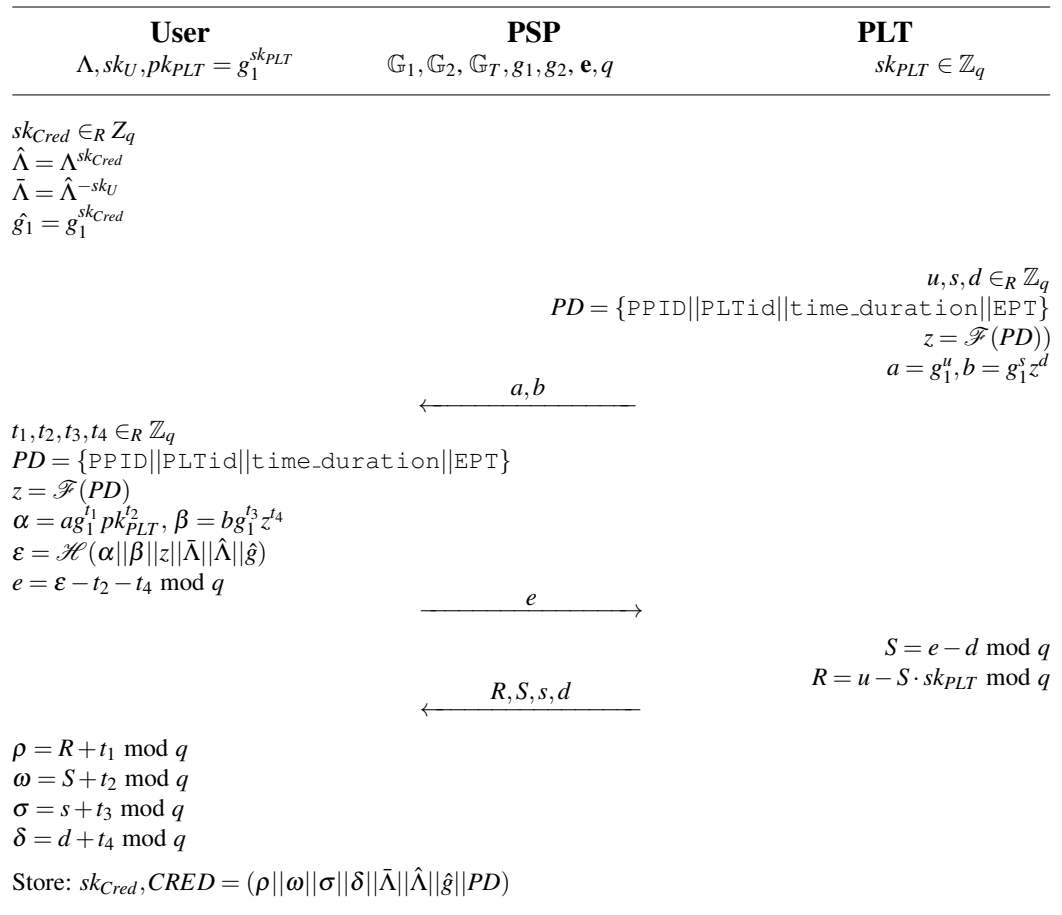
Figure 8 Issue algorithm.
