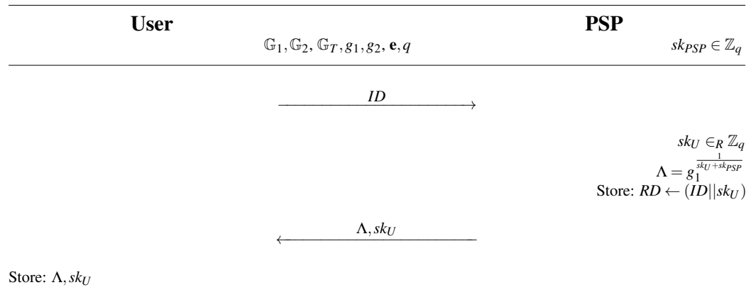
Figure 7 Register algorithm.
