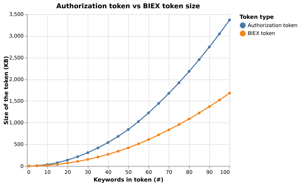
Figure 15 Token size.
