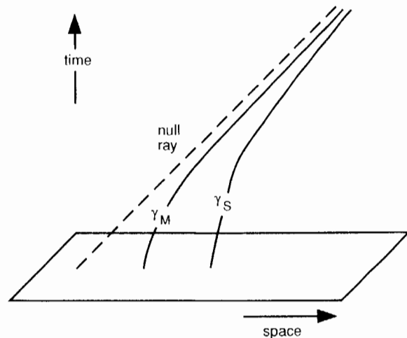
Figure 11.5 Slave and Master in Minkowski Spacetime
