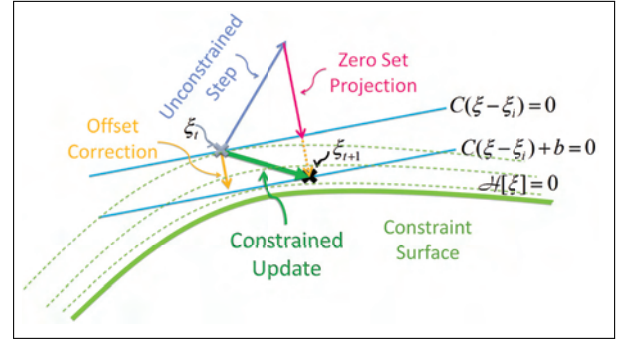
Fig. 8. The constrained update rule takes the unconstrained step and projects it with respect to A onto the hyperplane through \xi_t parallel to the approximated constraint surface (given by the linearization C(\xi - \xi_t) + b = 0 ). Finally, it corrects the offset between the two hyperplanes, bringing \xi_{t+1} close to \mathcal{H}[\xi] = 0 . (Image reproduced with permission from Dragan et al. (2011b).)
