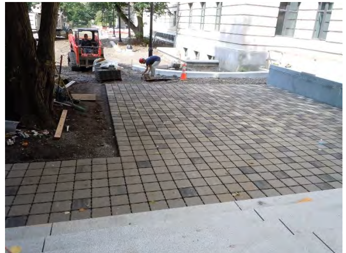
Permeable pavers were installed over the CU-Soil® and mature tree roots
