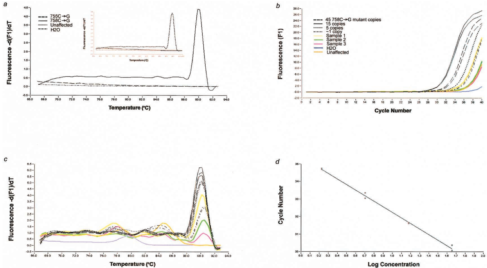
Figure 1 Specificity and sensitivity of the allele-specific PNA-PCRs. a , Melt-curve analysis after amplification of DNA from a patient with the 755C→G mutation yielded one specific peak. No cross reactivity with the other 758C→G mutation occurred. Inset shows melt-curve analysis for the 758C→G mutation with no cross reactivity for the 755C→G mutation. b , Amplification of standards and three samples of the 758C→G mutation. Standards used were 45, 15, 5, and 1 mutant copies diluted in human genomic DNA. Duplicates of each standard are shown. Negative controls are water and human genomic DNA. c , Melt-curve analysis after amplification of standards and samples from b . d , Standard curve for the 755C→G mutation with duplicates of each standard.
