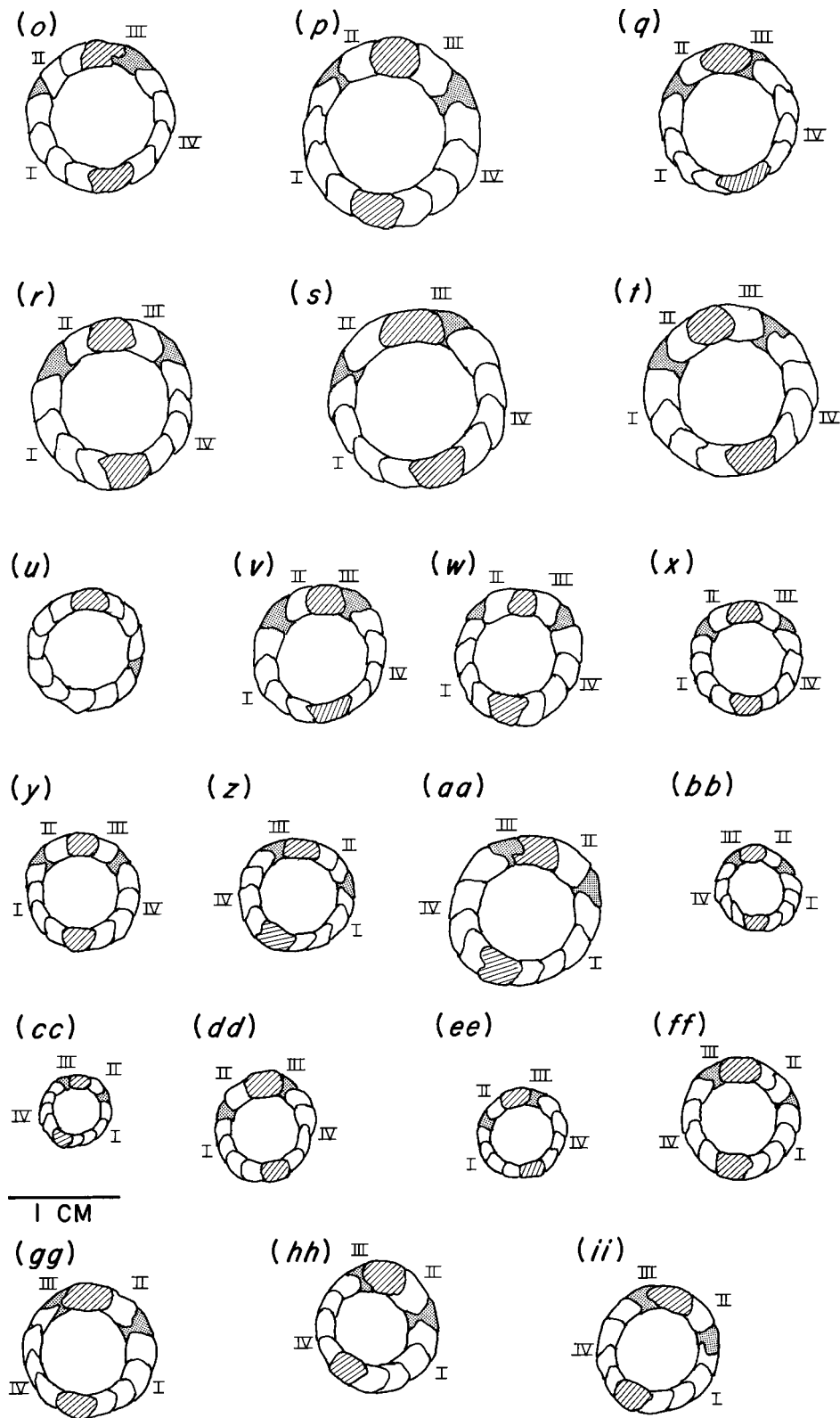
Figure 14. (o–ii). (o) Podica senegalensis (BMNH 1928.5.3.1); (p) Himantornis haematopus (AMNH 4183); (q) Porphyrio madagascariensis (UMMZ 227833); (r) Gymnocrex plumbeiventris (USNM 505787); (s) Habroptila wallacii (USNM 560792); (t) Aramides ypecaha (USNM 614590); (u) Amaurolimnas concolor (USNM 613961); (v) Rallina eurizonoides (AMNH 17718); (w) Cyanolimnas cerverei (USNM 343159); (x) Ortygonax sanguinolentus (USNM 227903); (y) Rallus longirostris (USNM 553301); (z) Nesoclopeus poecilopterus (BMNH 1940.12.8.82); (aa) Gallirallus okinawae (UMMZ 225360); (bb) Laterallus melanophaius (USNM 612029); (cc) Coturnicops novaboracensis (USNM 556931); (dd) Crex crex (USNM 490304); (ee) Porzana atra (USNM 562788); (ff) Amauornis olivaceus (USNM 560653; variant showing long segment II); (gg) Porphyriornis comeri (BMNH 1922.12.6.221); (hh) Gallinula [chloropus] cachinaans (USNM 347871); (ii) Fulica rufifrons (USNM 614603). See Appendix A for explanation of segments and nomenclature, Acknowledgments for institutional acronyms. In presumptive right rings, imbricated series progress in clockwise fashion; in
