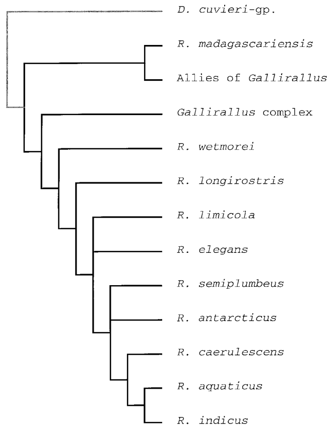
Figure 8. Single shortest tree recovered in a branch-and-bound analysis for modern species of Rallus ( sensu stricto ). Trees were rooted using Dryolimnas ; also included were ' Rallus ' madagascariensis and merged taxa representing Gallirallus (exclusive of torquatus -group) and allies of Gallirallus ( Tricholimnas , Nesoclopeus , Aramidopsis , Cabalus , Habropteryx and the ' G. ' torquatus -group). See table 1 and Appendix C for details concerning delimitation of terminal taxa.
