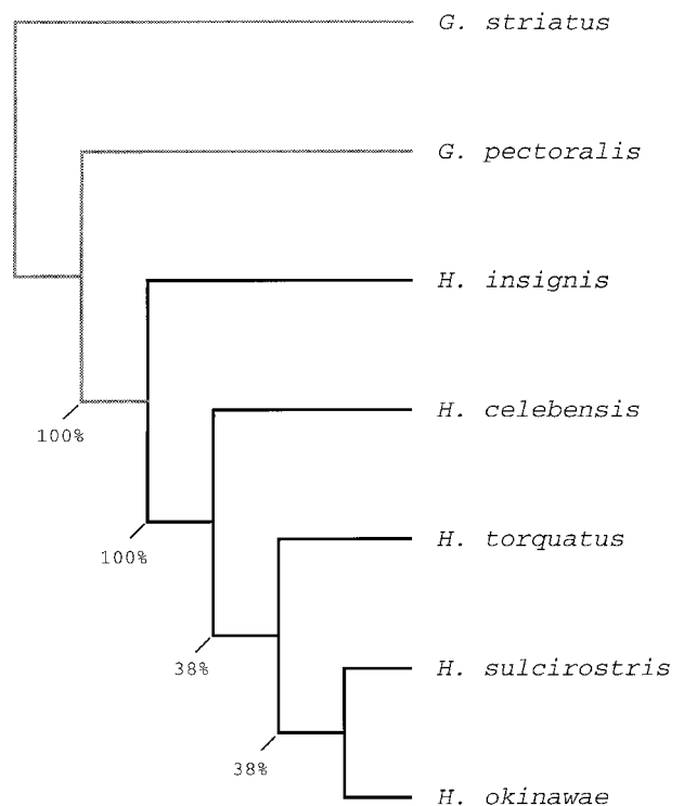
Figure 10. Majority-rule consensus tree for the eight shortest trees recovered in a branch-and-bound analysis of diagnosable partitions of the modern ' Gallirallus ' torquatus -group and ' G. ' okinawae , here labelled as congeneric with Habropteryx insignis . Trees were rooted using a paraphyletic series of closely related rallids; percentages are given for nodes conserved in the majority of the solution set and nodes compatible with the majority-rule nodes. See table 1 and Appendix C for details concerning delimitation of terminal taxa.
