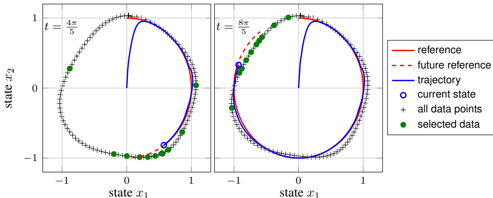
Figure 1: Snapshots of the desired and actual trajectory of the dynamical system. Data selected by Algorithm 1 lies close to the future reference and ensures a high tracking accuracy.
