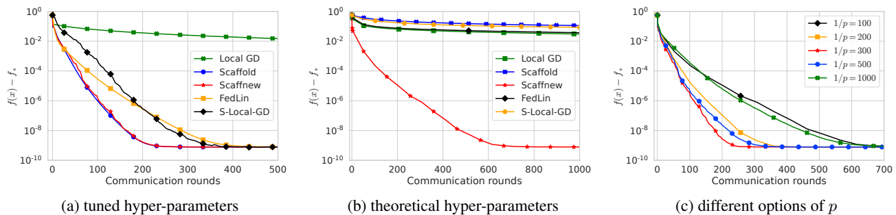
Figure 1. Deterministic Case. Comparison of Scaffnew to other local update methods that tackle data-heterogeneity and to LocalGD . In (a) we compare communication rounds with optimally tuned hyper-parameters. In (b), we compare communication rounds with the algorithm parameters set to the best theoretical stepsizes used in the convergence proofs. In (c), we compare communication rounds with the algorithm stepsize set to the best theoretical stepsize and different options of parameter p .
