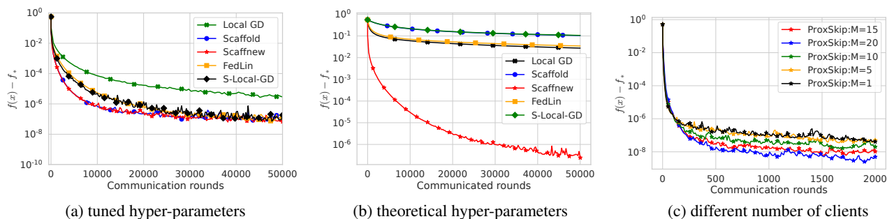
Figure 2. Stochastic Case. Comparison of Scaffnew to other local update methods that tackle data-heterogeneity and to LocalSGD . In (a) we compare communication rounds with optimally tuned hyper-parameters. In (b), we compare communication rounds with the algorithm parameters set to the best theoretical stepsizes used in the convergence proofs. In (c), we compare communication rounds with the algorithm parameters set to the best theoretical stepsizes used in the convergence proofs and different number of clients.
