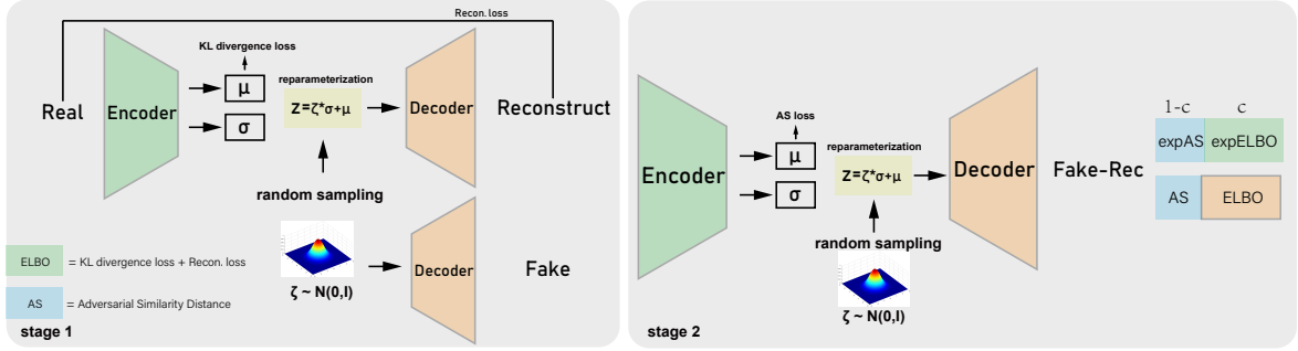
Figure 2: AS-IntroVAE workflow, using image reconstruction task as the example. AS-IntroVAE contains an encoder-decoder architecture. In the first phase, the encoder-decoder receives the real image and produce the reconstructed image. Meanwhile, the decoder will generate fake image from Gaussian noise alone. In the second phase, the same encoder-decoder conduct adversarial learning in the latent space for the reconstructed image and the fake image. During adversarial learning, the encoder tries to maximize the adversarial similarity distance between fake image and reconstruction image, whereas the decoder wants to minimize it. After each iteration, the model will calculate the annealing rate c .
