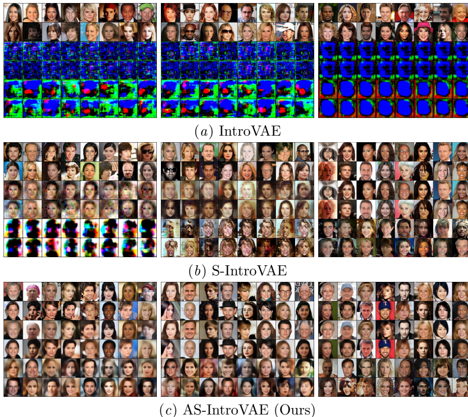
Figure 7: The training stability visual comparison at CelebA-128 dataset. From left to right panel: 10 epoch, 20 epoch, 50 epoch. For each image grid, the first and the second row are real images, the third and fourth rows are reconstructed images, and the fifth and sixth rows are generated images. Zoom in for a better view.
