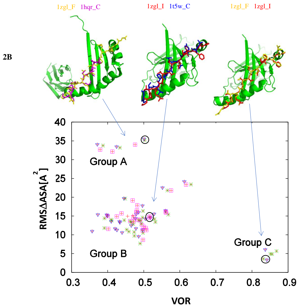
Fig. 2. Comparison of partner interface surface differences with MoRF chain overlap. (A) Plot of RMS \Delta ASA versus backbone VOR for Dataset_160, with representative cartoons showing partners (green ribbons) and MoRF pairs (red and blue sticks) for various points in the plot. Arrows and black circles indicate the locations of these structure pairs in the plot. (B) Plot of RMS \Delta ASA versus backbone VOR for an example cluster, the HLA-DR2A cluster (cluster ID 57). Representative cartoons showing partners (green ribbons) and MoRF pairs (sticks with other colors) for each labeled group of pairs (groups A, B, and C) show the main differences between the three groups. Actual points on plot where representative cartoons were made are marked with a black circle.
