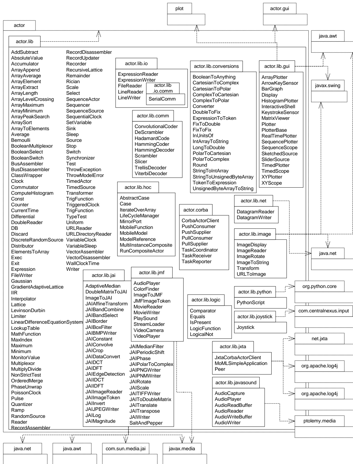
FIGURE 1.18. The major actor libraries are in packages containing domain-polymorphic actors (not complete).
