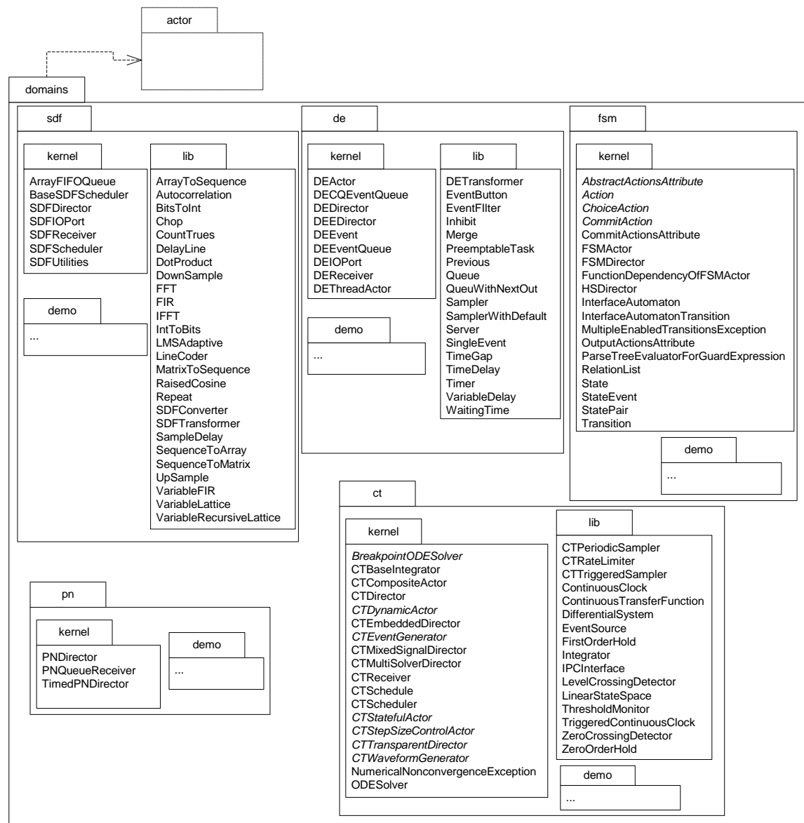
FIGURE 1.17. Package structure of some of the Ptolemy II domains.
