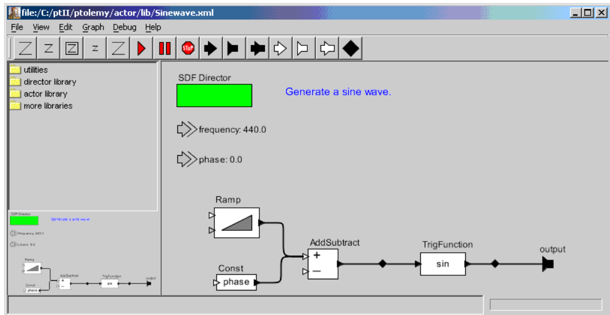
FIGURE 7.12. Rendition of the Sinewave class in Vergil 1.0.
