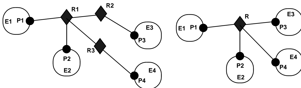
FIGURE 7.5. A relation group is maximal set of linked relations. At the left, R1, R2, and R3 form a relation group. A relation group is semantically identical to a single relation, so the two diagrams above have the same meaning.
