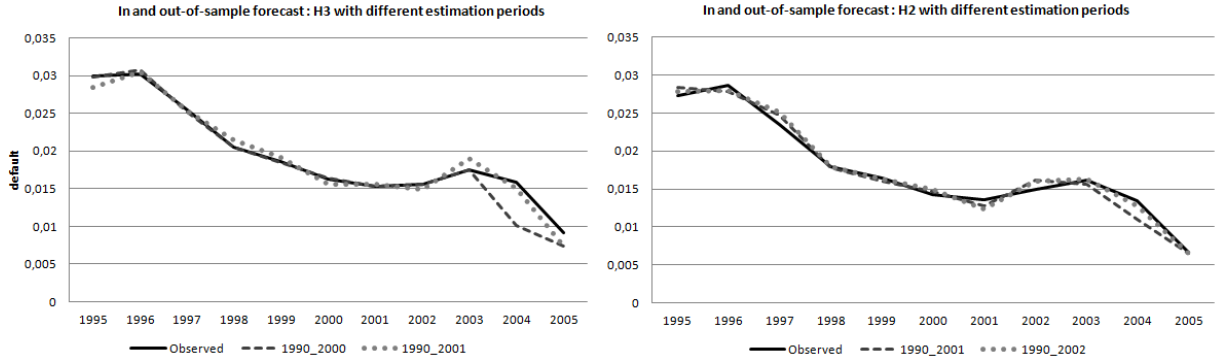
Figure 7: In- and out-of-sample performance of Model III (H3 and H2) without spline method. This figure displays in- and out-of-sample forecast of the aggregate bankruptcy rate. For each case (H=3 or H=2), the observed rate (black solid line) is compared with the performance of two multi-period Logit models. In the case H=3 (left-hand sub-figure), the models are estimated on the period 1990-2000 (black dashed line) and 1990-2001 (grey dotted line). In the case H=2 (right hand subfigure), the models are estimated on the period 1990-2001 (black dashed line) and 1990-2002 (grey dotted line).
