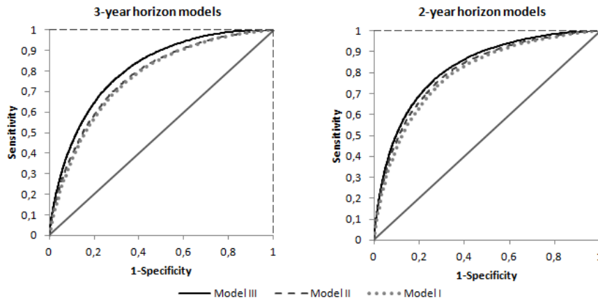
Figure 6: ROC curves. This Figure displays ROC (Receiver Operating Characteristic) curves of different specifications of Logit model : model I, II and III and for the case "H=3" and "H=2". The area under the ROC curve (AUC) is a measure of how well a model can distinguish between two groups : bankrupted/non- bankrupted (see Tables 1 and C).
