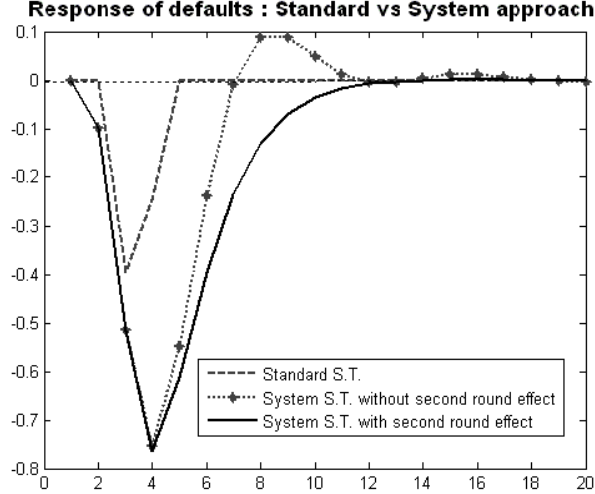
Figure 4: Comparison of stress testing (S.T.) exercises. This Figure displays different impulse responses of defaults to a positive one standard deviation shock on the output gap with different stress test (S.T.) approaches namely, "Standard S.T" (single equation: first equation of system (B)), "System S.T. with second round effect" (running dynamically the whole system (B), as in Figure 3) and "System S.T. without second round effect" (running dynamically the constrained system (B) with a_2 = 0 ).
