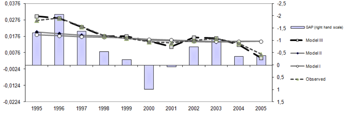
Figure 5: Aggregate bankruptcy rate observed and estimated at t for the case "H=2". 32 This figure displays the negative relationship between the output gap (GAP, with inverted scale) and the bankruptcy rate estimated by model III (black long dashed line with box), which is closer to the observed rate (black short dashed line with triangle) than the one estimated by model II (grey solid line with diamond) or model I (grey solid line with box). See results in Table C.
