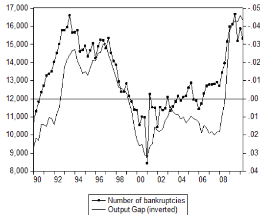
Figure 1: Number of bankruptcies and the output gap in France (1990-2010). Source: Banque de France.
