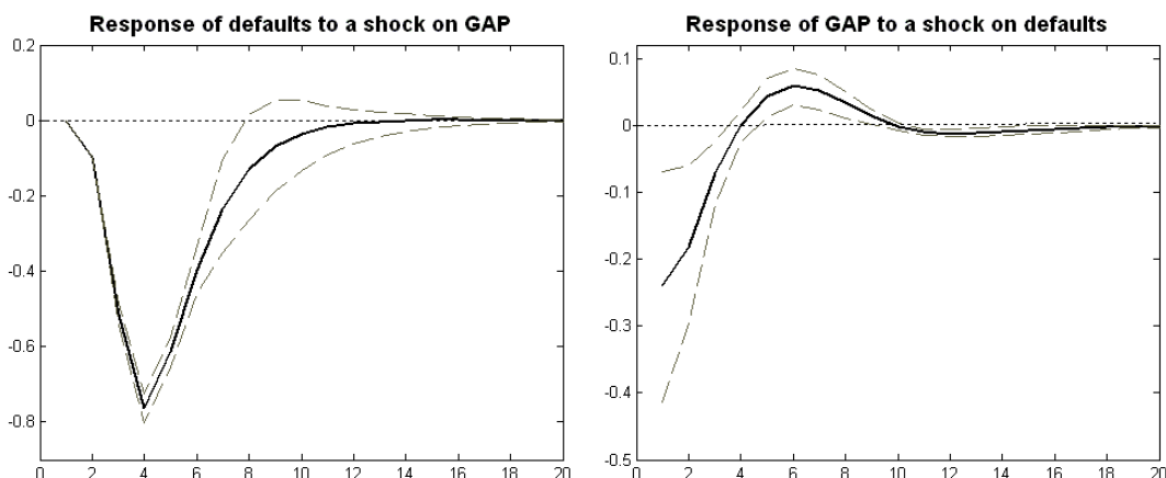
Figure 3: Impulse Response Function from Panel VAR (%)—black solid line, with Monte Carlo confidence intervals at 90%, 1000 Trials (dashed grey lines). The Figure displays the response of the default ratio and the output gap to a positive one standard deviation shock to the GAP, including the effect of the initial shock to the GAP on the additional macroeconomic variables (INF, IRL). The simulation of our system (B) of two equations allows us to consider second round effects.
