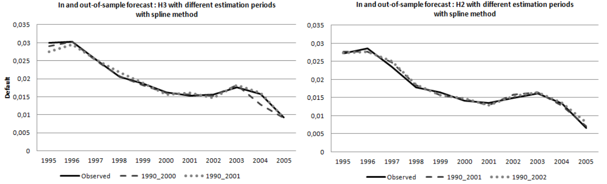
Figure 8: In- and out-of-sample performance of Model III (H3 and H2) with spline method. This figure displays in- and out-of-sample forecast of the aggregate bankruptcy rate. For each case (H=3 or H=2), the observed rate (black solid line) is compared with the performance of two multi-period Logit models, which include spline transformations of macroeconomic variables. In the case H=3 (left-hand sub-figure), the models are estimated on the period 1990-2000 (black dashed line) and 1990-2001 (grey dotted line). In the case H=2 (right hand subfigure), the models are estimated on the period 1990-2001 (black dashed line) and 1990-2002 (grey dotted line).
