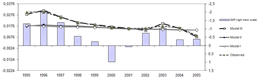
Figure 2: Aggregate bankruptcy rate observed and estimated at t for the case "H=3". The Figure displays the negative relationship between the output gap (GAP, with inverted scale) and the bankruptcy rate estimated by model III (black long dashed line with box), which is closer to the observed rate (black short dashed line with triangle) than the one estimated by model II (grey solid line with diamond) or model I (grey solid line with box). See results in Table 1.
