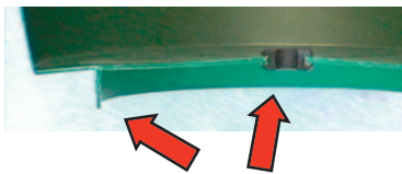
Cross section showing reinforced support ring and reinforced grommet area of our medium and large rebar bowls.
