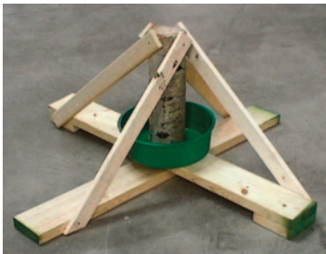
48" 2x6 with braces and Bowl 10Q
