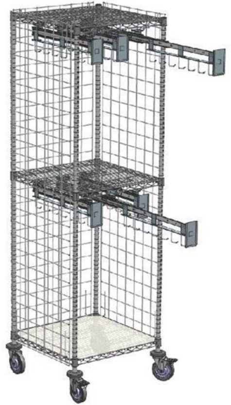
Pull-Out Catheter Slide Modules For Your Existing Shelving Units. 18" Unit Has (5) Hooks & 24" Units Has (7) Hooks. 18"-MMUSC18 24" - MMUSC24
