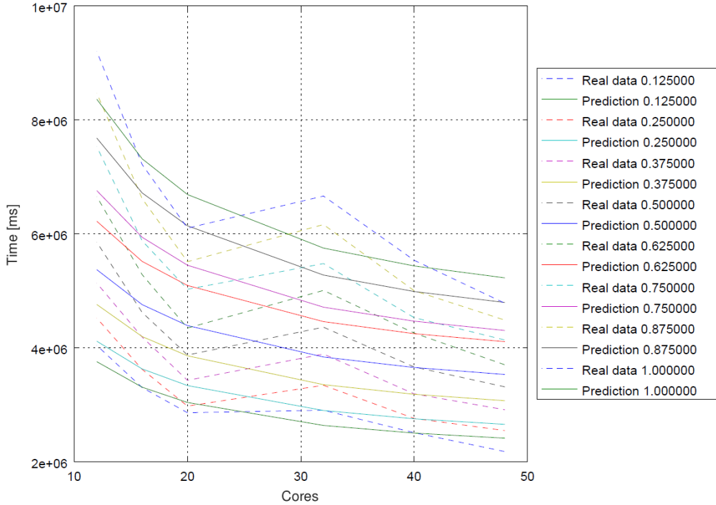
Figure 3: Predicted Regression Curves of the Confidence Model.
