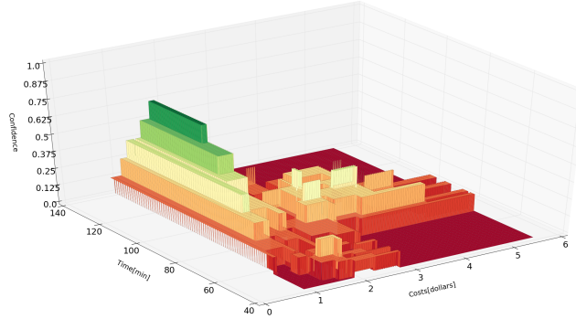
Figure 7: Scenario 1: comparison between the two pricing policies.
