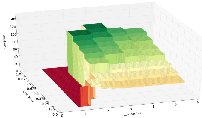
Figure 9: Time minimization with discrete hourly cost.
