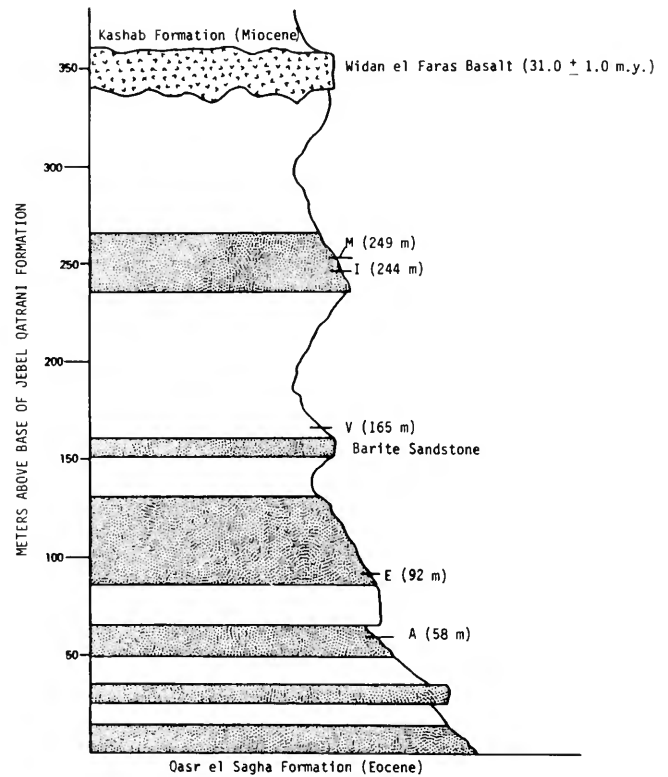
FIGURE 2.—Simplified section of the Jebel Qatrani Formation showing the stratigraphic positions of quarries that have produced birds. The sediments lying above the Barite Sandstone constitute the upper sequence, those below constituting the lower sequence. The vast majority of bird specimens have come from Quarries I and M of the upper sequence. Quarry V has not yet produced any diagnostic bird elements. Quarries E and A have each produced a single diagnostic bone (of a jacanid and accipitrid, respectively). Modified from Bown and Kraus (1987).
