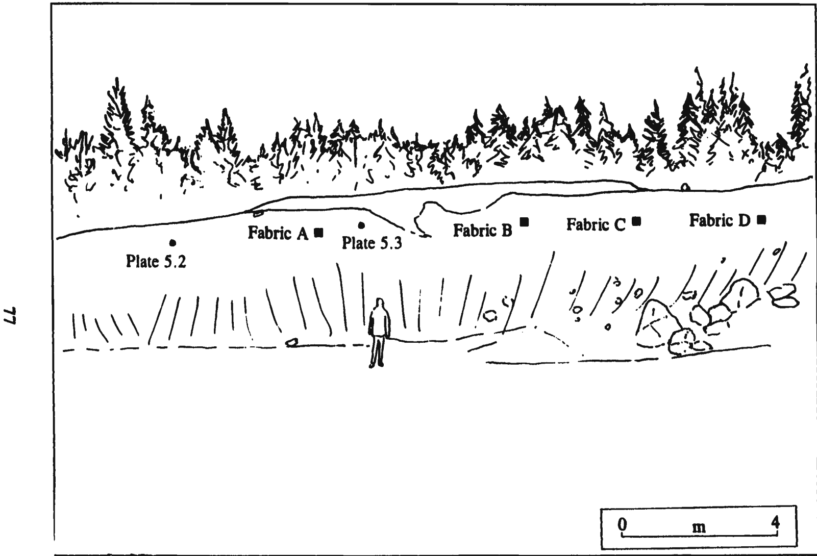
Figure 5.2 - Clast fabric analysis sites in Section A11a and the location of Plates 5.2 and 5.3.
