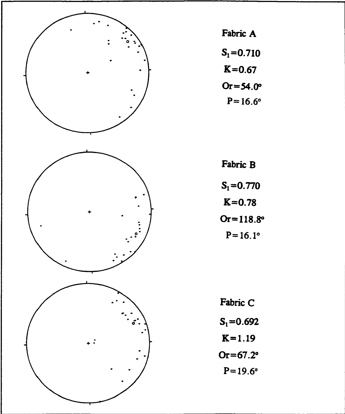
Figure 6.4 - Stereoplots of fabrics measured at Section A9.
