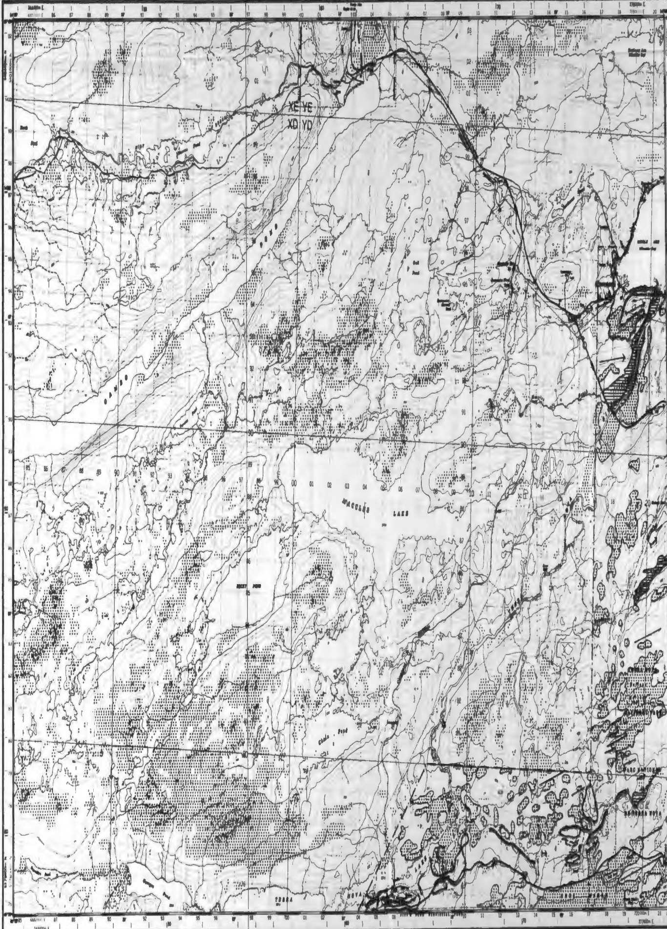
Figure 4.1 - Geomorphology of the Glovertown map sheet (NTS 2 000)
