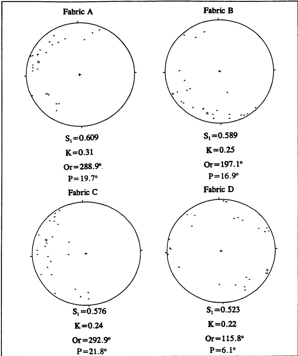
Figure 5.3 - Stereoplots of fabrics used to determine ice flow direction at Section A11a.
