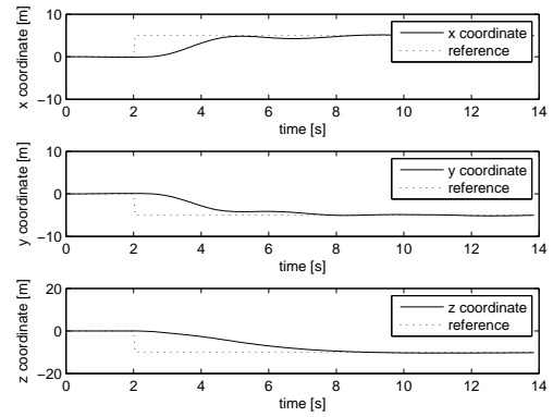
Fig. 3. Position control of the vehicle using LQR
