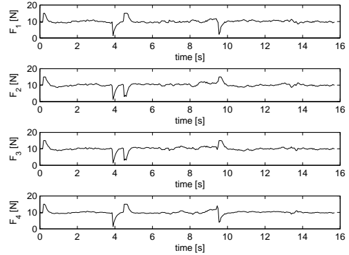
Fig. 9. Control Effort in Sliding Mode Controller
