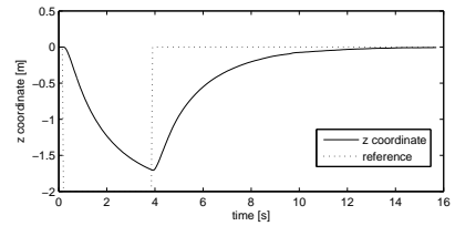
Fig. 8. Altitude Control Using Sliding Mode Controller
