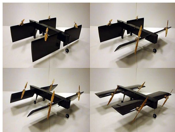
Fig. 1. SUAVI with integrated actuators in different flight configurations
