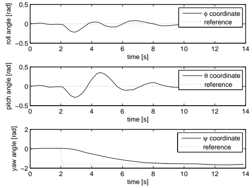
Fig. 4. Attitude control of the vehicle using LQR
