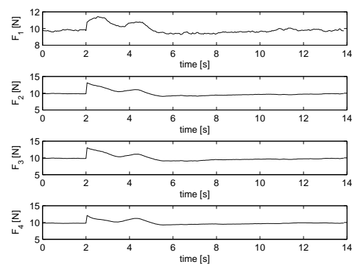
Fig. 5. Forces generated by the motors
