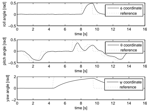
Fig. 7. Attitude Control Using Sliding Mode Controller
