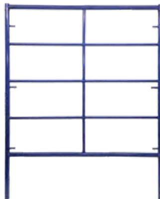
SWS-LFTDB56.4 5'X6'4" DOUBLE BOX TRIPLE LADDER WT. 51.80 LBS
