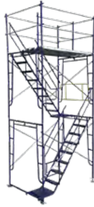
SWS-NRST-13 13FT STATIONARY SCAFFOLD STAIR TOWER WT. 727.68 LBS
