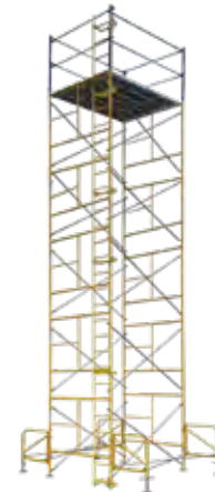
SWS-NRT-25L 25FT STATIONARY SCAFFOLD TOWER WITH ACCESS LADDER WT. 933.87 LBS
