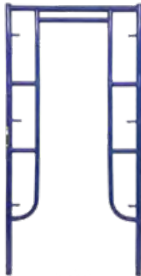
SWS-WT426.4 42"X6'4" WALK THRU FRAME WT. 40.00 LBS
