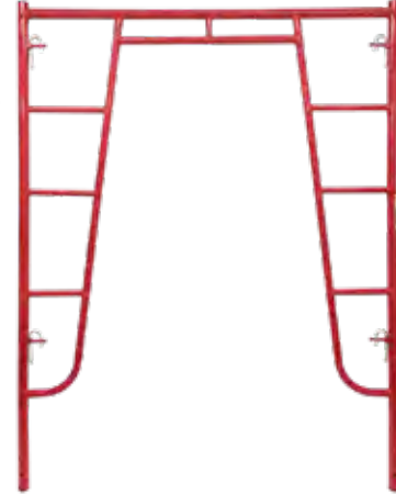
SWS-WT56.7 5'X6'7" WALK THRU FRAME WT. 45.56 LBS
