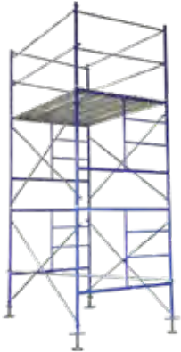
SWS-NRT-10 10FT STATIONARY SCAFFOLD TOWER WT. 424.89 LBS
