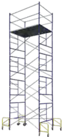
SWS-RT-20 20FT ROLLING SCAFFOLD TOWER W/OUTRIGGERS WT. 638.48 LBS
