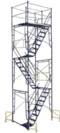
SWS-NRST-20 20FT STATIONARY SCAFFOLD STAIR TOWER W/OUTRIGGERS WT. 1106.78 LBS
