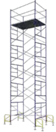
SWS-NRT-25 25FT STATIONARY SCAFFOLD TOWER W/OUTRIGGERS WT. 748.29 LBS
