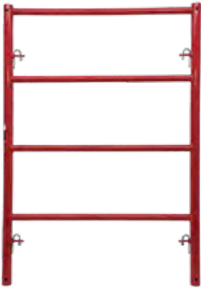
SF4X6 4'X6' SHORING FRAME WT. 65.20 LBS
