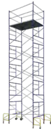
SWS-RT-25 25FT ROLLING SCAFFOLD TOWER W/OUTRIGGERS WT. 749.28 LBS
