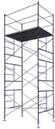
SWS-NRT-15 15FT STATIONARY SCAFFOLD TOWER WT. 532.69 LBS
