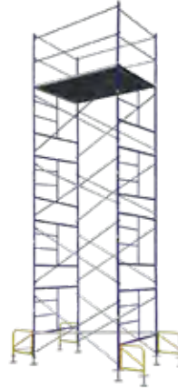
SWS-NRT-20 20FT STATIONARY SCAFFOLD TOWER W/OUTRIGGERS WT. 640.49 LBS
