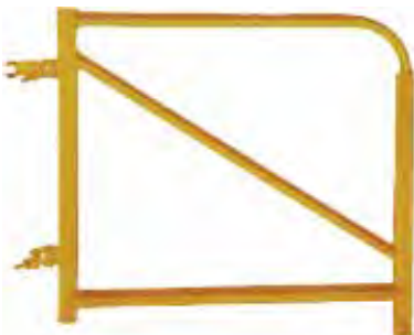
SWS-OR30 30" OUTRIGGER FOR FRAME SCAFFOLD WT. 18.80 LBS
