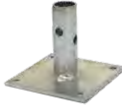
SWS-BP13/8 1-3/8" STEM W/BJ STYLE 5"X5" BASE PLATE WT. 1.91 LBS
