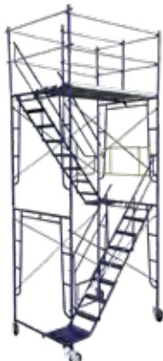
SWS-RST-13 13FT SCAFFOLD STAIR TOWER WT. 770.87 LBS
