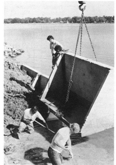
Figure 17. Precast concrete modules can be used in low energy situations to build bulkheads.
