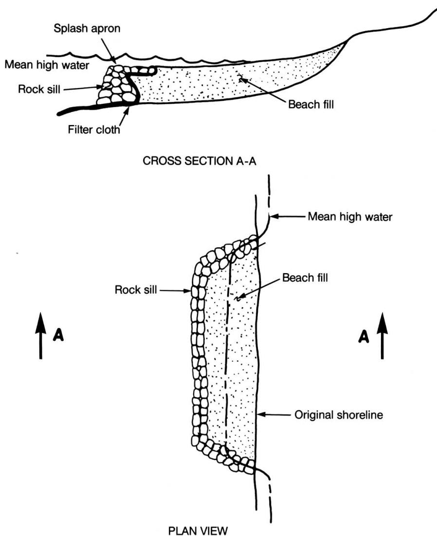
Figure 31. A perched beach is held in place by a submerged dike or sill on its seaward side. This form of protective beach is more expensive than simple renourishment. (Adapted from U.S. Army Corps of Engineers 1981.)
