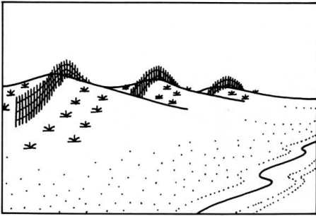
Figure 32. Snow fence can be used to trap windblown sand and “build” a dune to protect inland areas. Such dunes should then be stabilized with vegetative plantings.
