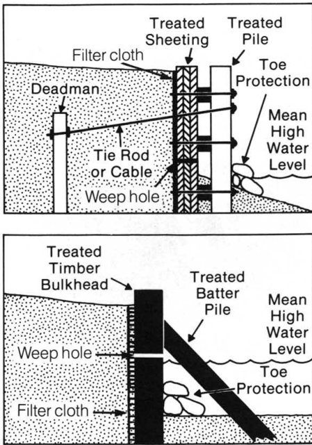
Figure 18. Treated-timber bulkheads rely on either deadmen or bracing for additional structural strength. Untreated wood will deteriorate rapidly in a marine setting.
