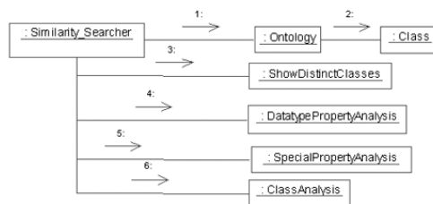
Fig. 6. Similarity_Searcher collaborates with other objects to find similarities.
