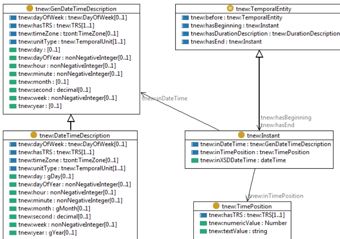
Figure 2 – Generalized time ontology for supporting additional temporal position encodings.
