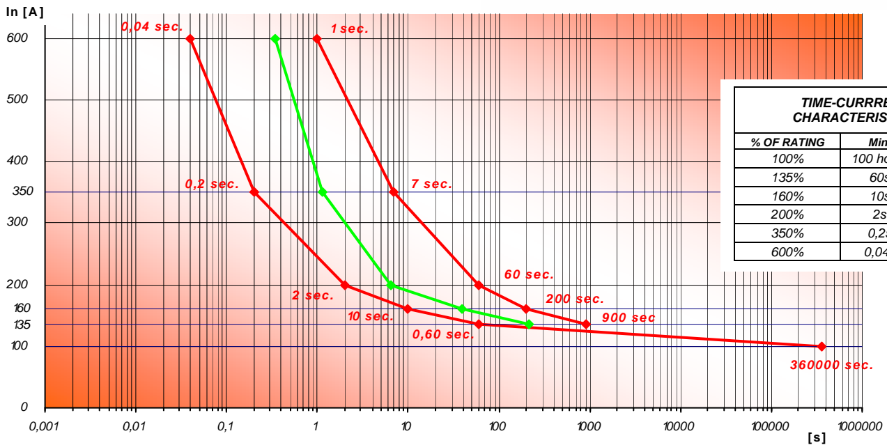
Example Fuse time-current curve (FORM E 40A) :
