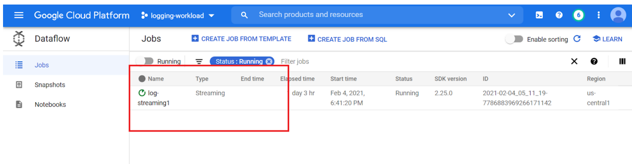
Figure 24. Dataflow job.
