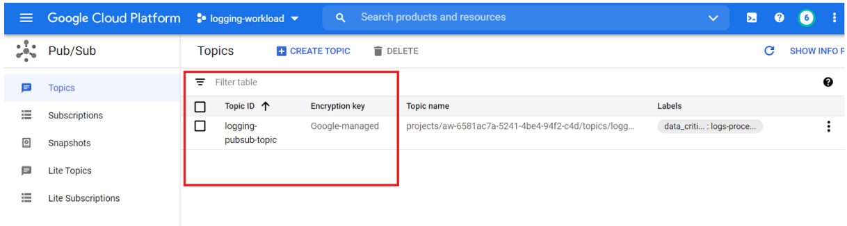
Figure 22. Pub/Sub topic.
