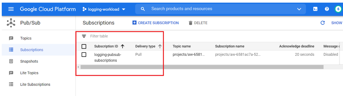
Figure 23. Pub/Sub subscription.
