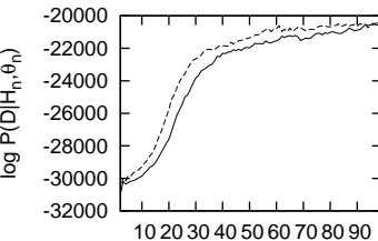
Discrete HMM
