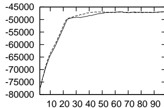
Gaussian HMM
