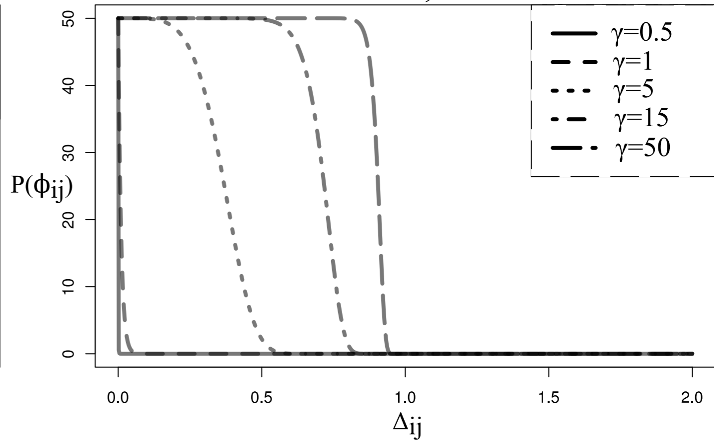
Prior curve, \lambda=0.01
