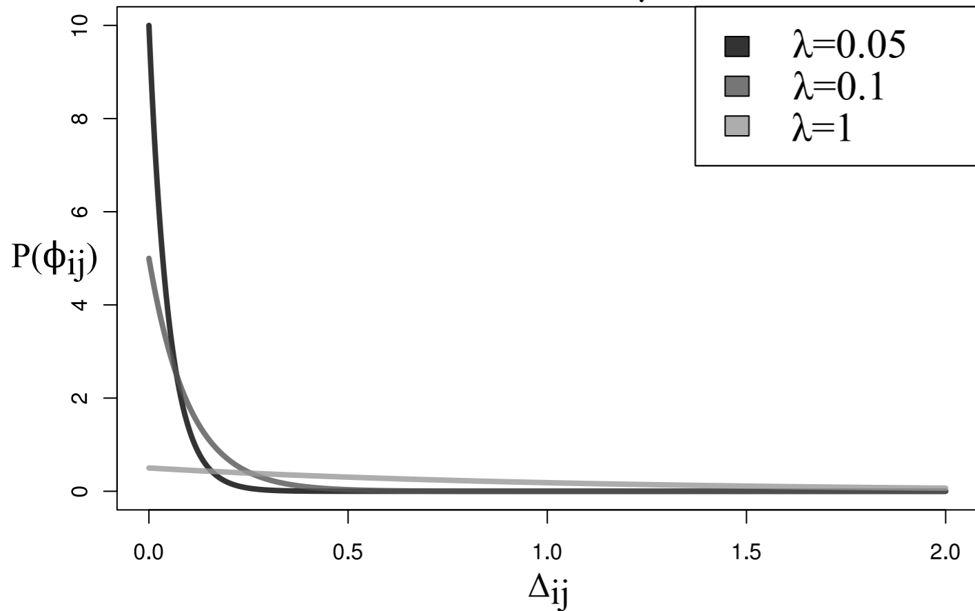
Prior curve, \gamma=1
