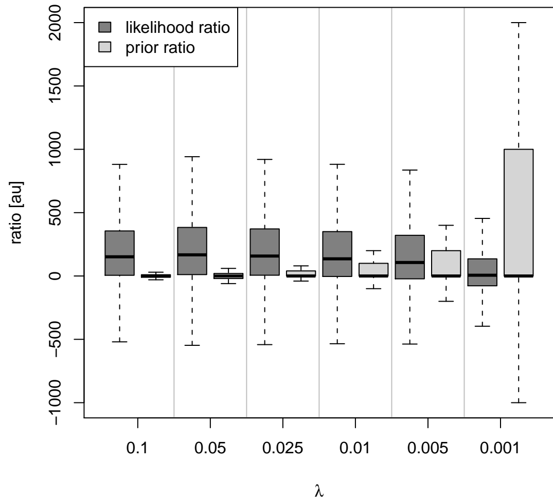
comparison prior and likelihood ratios
