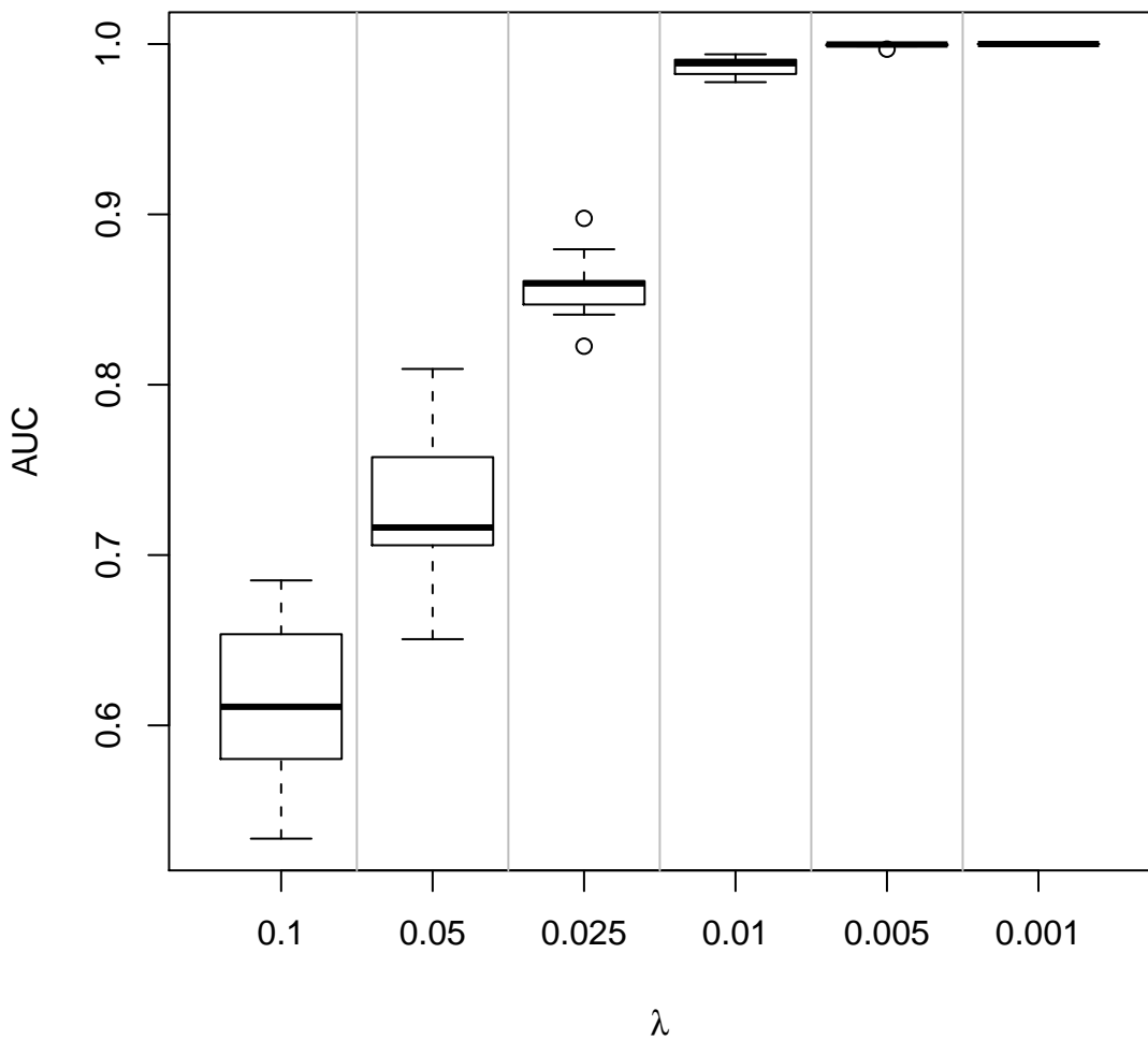
AUCs for 10 reconstructions
