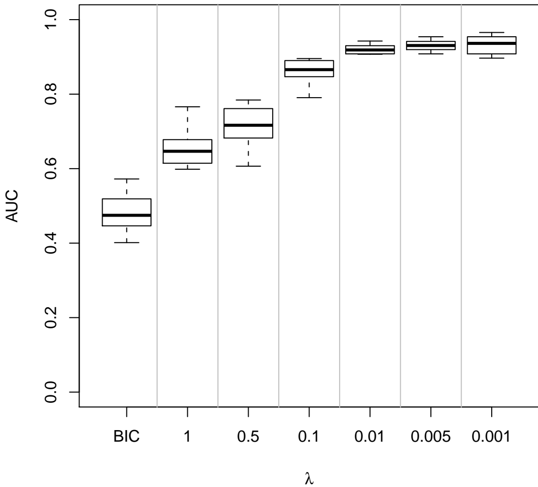
AUCs for 10 reconstructions GA, laplace prior
