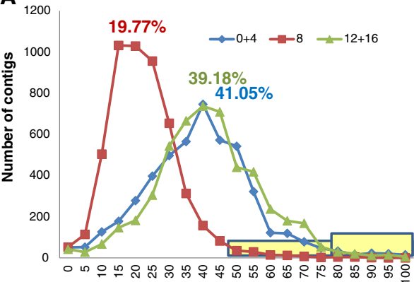
Distribution of percent of contig reads observed in specified age group
