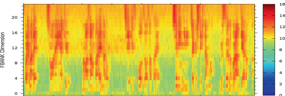
(B) Reverberant feature vectors, Y(t) .
