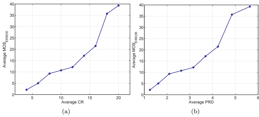
Fig. 15: The clinical evaluation of the proposed compression algorithm by means of MOS_{ERROR} , CR, and PRD: (a)The variation of the average MOS_{ERROR} with respect to the CR; (b)The variation of the average MOS_{ERROR} with respect to the PRD
