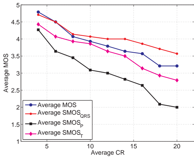
Fig. 17: The variation of the average MOS, SMOS_{QRS} , SMOS_T , and SMOS_P with respect to the CR
