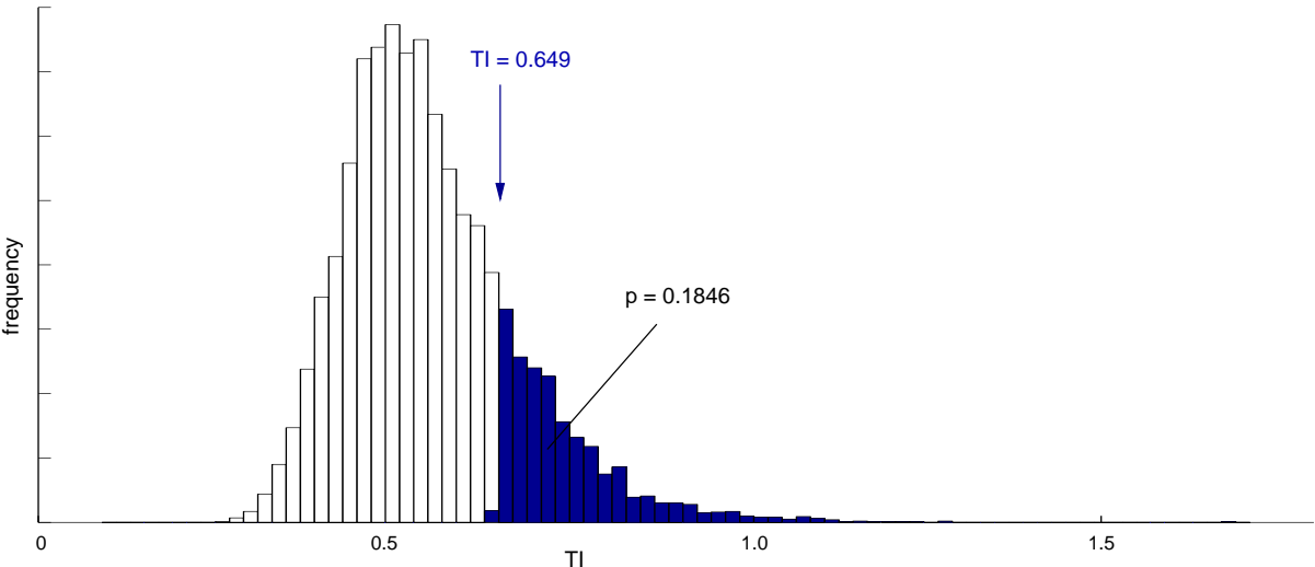
TI distribution of random trees
