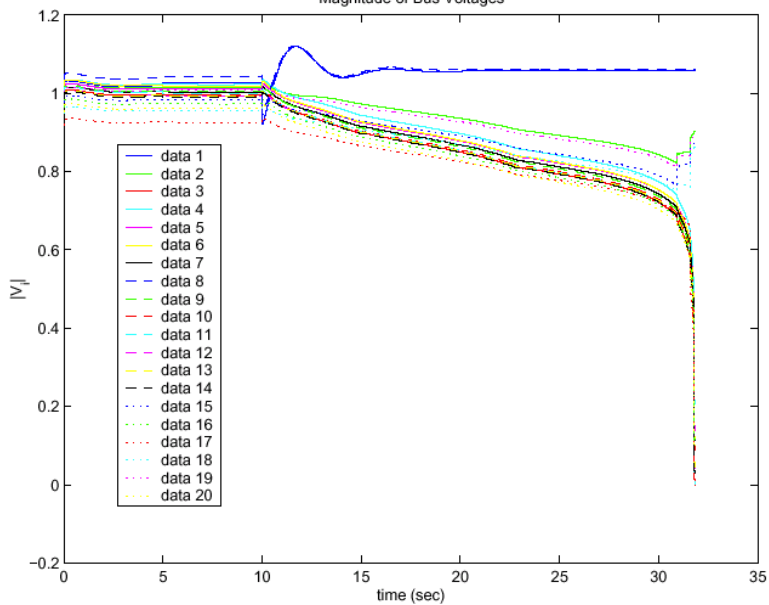
Magnitude of Bus Voltages
