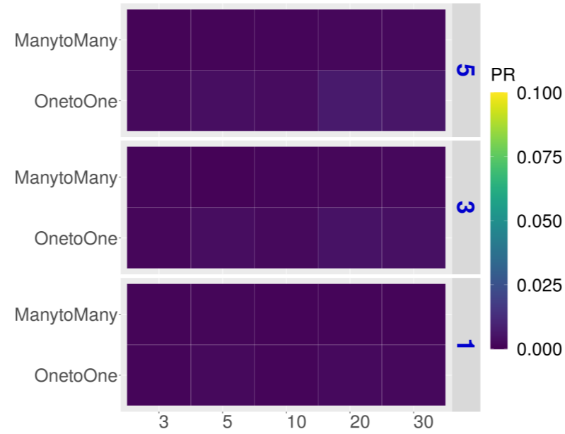
Halpern's Score (P-value)
