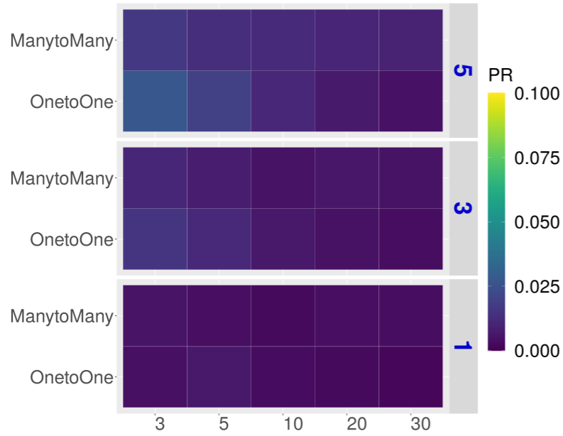
Sum Score (P-value)
