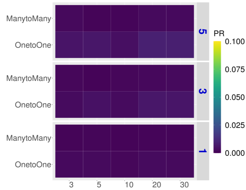
Halpern's Score (P-value)
