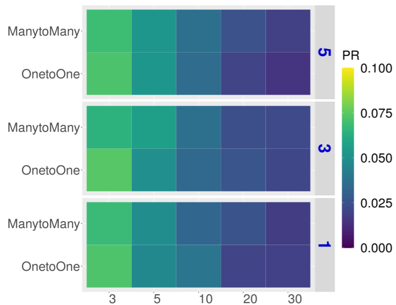
Product Score (P-value)
