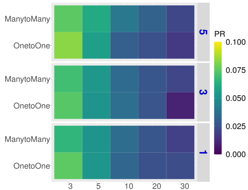
Product Score (P-value)
