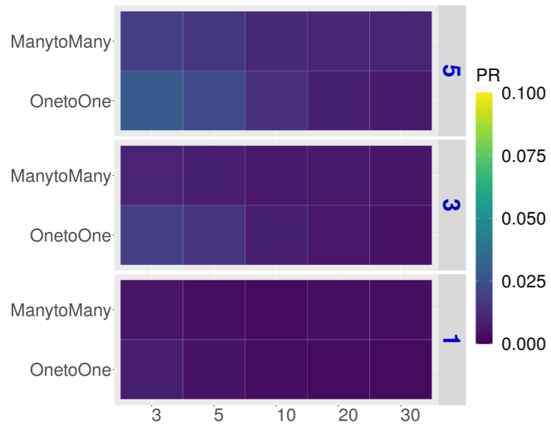
Sum Score (P-value)
