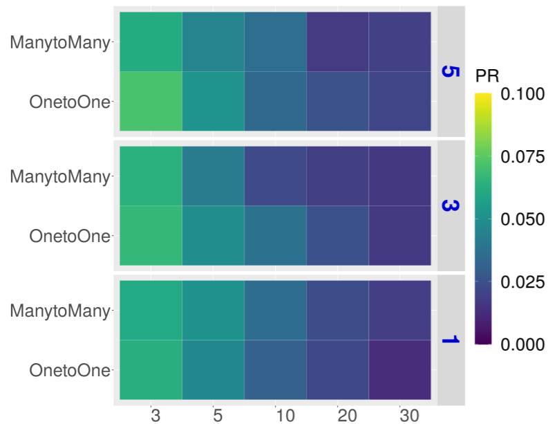
Product Score (P-value)
