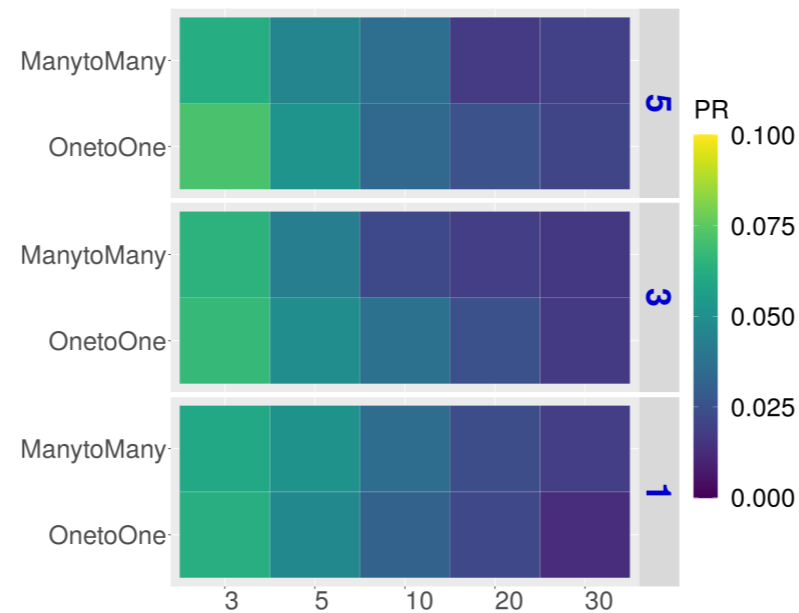
Cabello-Aguilar's Score (P-value)
