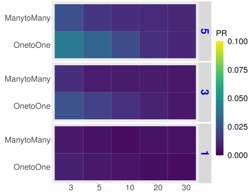
Sum Score (P-value)
