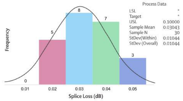
Fig.11 Splice loss of G.657A1 - G.657A2 fibre at 1310 nm
