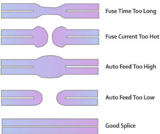
Fig. 3 Fibre end conditions
