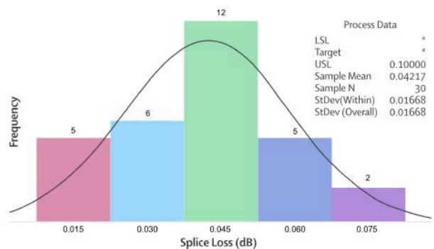
Fig. 7 Splice loss of G.652.D - G.657.A1 fibre at 1310 nm
