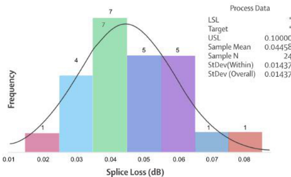
Fig. 10 Splice loss of G.652.D - G.657A2 fibre at 1550 nm
