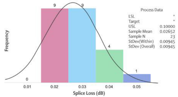
Fig.12 Splice loss of G.657A1 - G.657A2 fibre at 1550 nm
