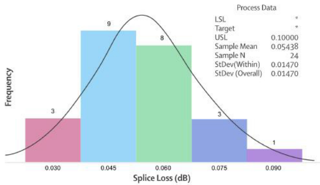
Fig. 9 Splice loss of G.652.D - G.657A2 fibre at 1310 nm
