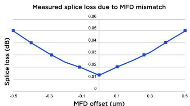
Fig. 2 Measured splice loss as a function of MFD mismatch
