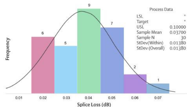
Fig.8 Splice loss of G.652.D - G.657.A1 fibre at 1550 nm
