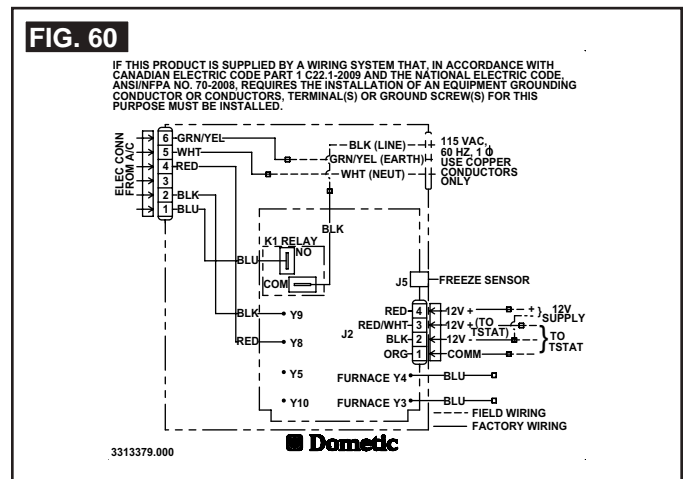
2. 3313189.000 & 3313189.015 LCD SZ Electronic Control Kit Wiring Diagram Cool/Furnace
