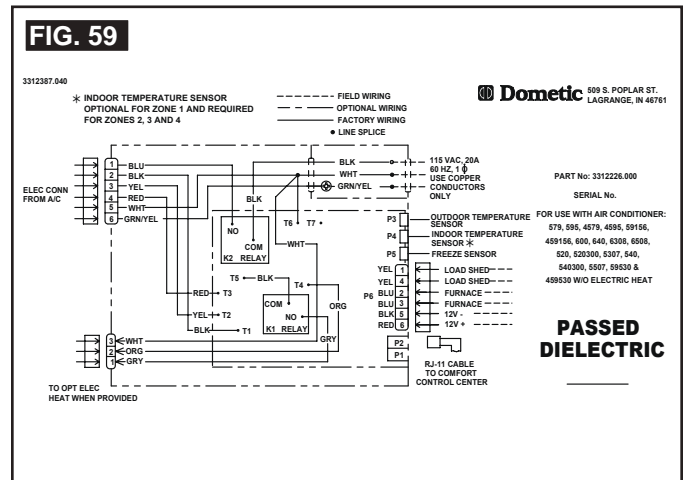
1. 3312020.000 CCC 2 Electronic Control Kit Wiring Diagram
