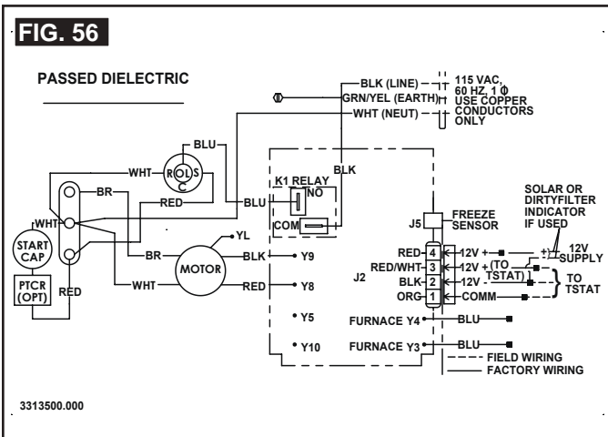
10. 641915 & 641916 Unit Wiring Diagram
