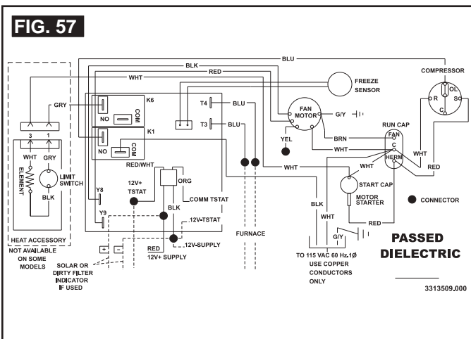
11. 641935 Unit Wiring Diagram
