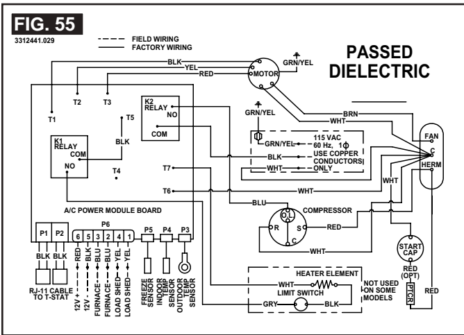
9. 541815, 541816, 641815, 641816 & 641835 Unit Wiring Diagram
