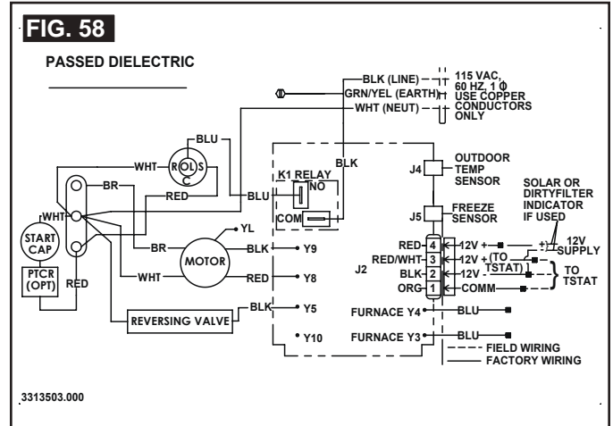
12. 651916 Unit Wiring Diagram
