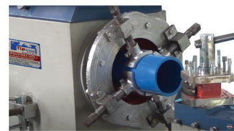
PVC Clamping Arrangement
