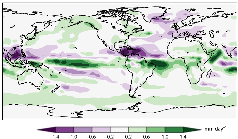
FIGURE 16. Annual-mean precipitation change resulting from a CO 2 doubling and AMOC breakdown. Most concerning is the southward shift in tropical rainfall belts and a generally drier Europe. From Liu et al. (2017)
