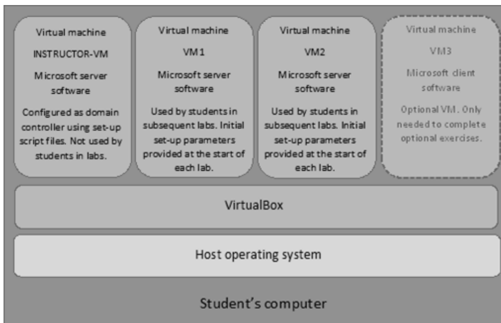
Figure 2: Virtualisation abstraction on a student's computer
