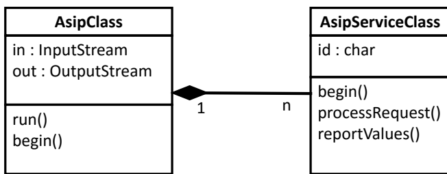
Figure 1: ASIP simplified class diagram
